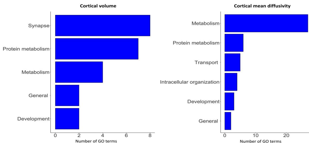
Figure 5 Total number of GO biological process terms negatively associated with cortical cell loss in premanifest Huntington's disease. Each row represents the number of GO terms involved within the module. GO = gene ontology.
