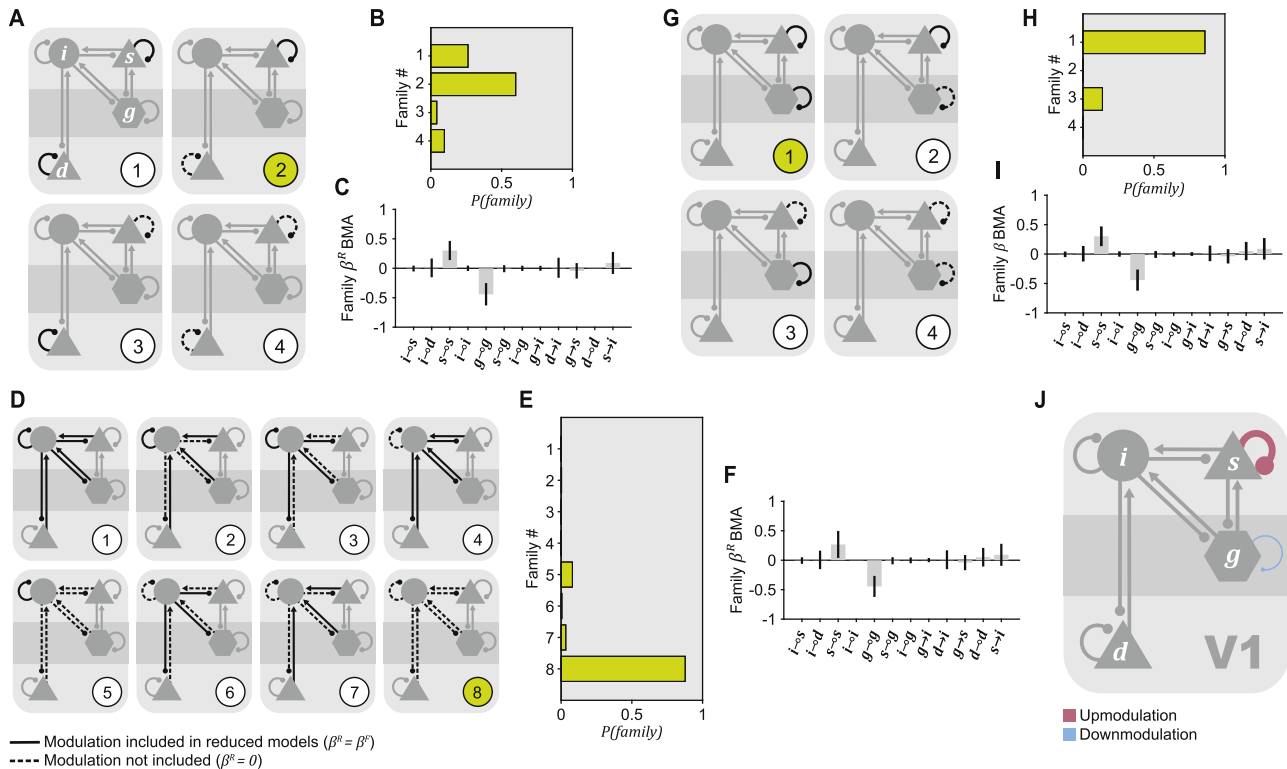
Fig. 4. The role of inhibition in attentional modulation. (A–C) Hypotheses about the role of pyramidal population self-inhibition in the supragranular and deep layers. (A) Schematic representation of the four hypotheses shown on an exemplar V1 microcircuit. Connections shown in continuous black lines are modulated by attention, connections shown in dashed black lines are not significantly modulated, whereas connections shown in grey may or may not be modulated. (B) Posterior probability of each family corresponding to a hypothesis shown in A. The index of the family with the highest posterior probability is highlighted with green in A. (C) BMA of the attentional modulation \beta^R across all reduced models that belong to the winning family. (D–F) Same as A–C, but for hypotheses about the modulation of input or response gain of the inhibitory population. (G–I) Same as A–C, but for hypotheses about the role of self-inhibition in the supragranular pyramidal and in the granular population. (J) Schematic representation of the results shown in G–I, specifically the “attend in” over the “attend out” connection strength ratio for connections significantly modulated with attention. Conventions as in Fig. 3F. Here, the significance of attentional modulation for each connection is considered relative to the BMA of \beta^R .
