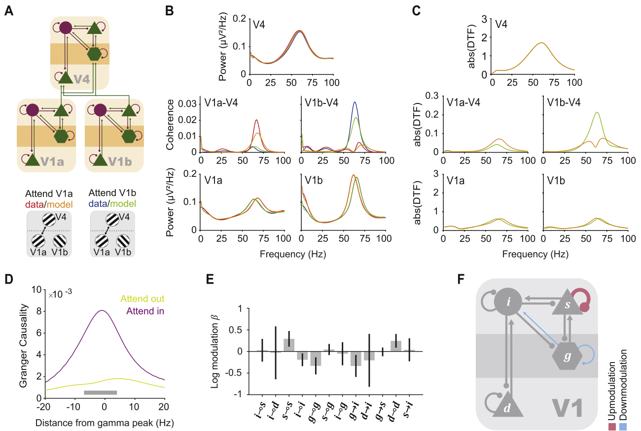
Fig. 5. Attentional modulation in the no-feedback architecture. (A) Top : Schematic representation of the V1a-V1b-V4 microcircuit without V4-to-V1 feedback. Bottom : Legend for panels B-C. (B) Power spectral density and coherence spectra averaged across the 10 V1a-V1b-V4 triplets of monkey P. (C) Absolute DTFs averaged across the 10 V1a-V1b-V4 DCMs of monkey P. (D) GC from V1 to V4 in the fitted models, as a function of frequency relative to the individual gamma peak frequency of the respective monkey. Conventions as in Fig. 3D. (E) PEB posterior estimate combining data from both monkeys. Conventions as in Fig. 3E (F) Schematic representation of the BMA of the attentional modulation \beta within the family of reduced models with the highest posterior probability (in which \beta_{s \rightarrow s}^R = \beta_{s \rightarrow s}^F , \beta_{g \rightarrow g}^R = \beta_{g \rightarrow g}^F and \beta_{g \rightarrow i}^R = \beta_{g \rightarrow i}^F ). Conventions as in Fig. 3F.
