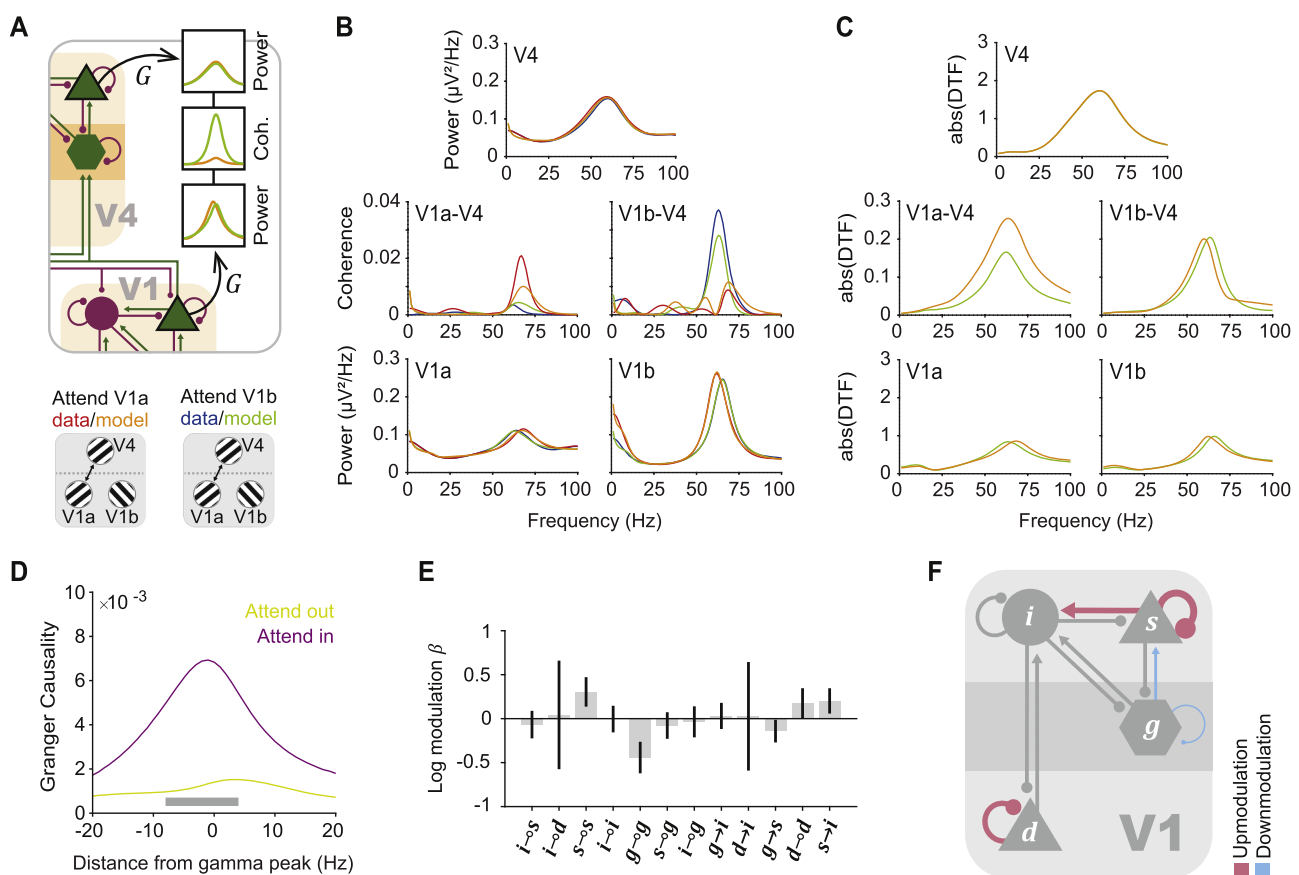
Fig. 3. DCM of the attentional effects. (A) Top : Schematic representation of the observation model used in the present study: The LFP of a node consists of the depolarization of the respective supragranular pyramidal population, weighted by the parameters of the observation model G . Bottom : Legend for panels A-C. (B) Power spectral density and coherence spectra averaged over the 10 V1a-V1b-V4 triplets of monkey P. Top : V4 power spectrum, bottom : V1a and V1b power spectra, middle : V1a-V4 and V1b-V4 coherence spectra. (C) Absolute DTF averaged over the 10 V1a-V1b-V4 DCMs of monkey P. (D) GC from V1 to V4 in the fitted models, as a function of frequency relative to the individual gamma peak frequency of the respective monkey, averaged over V1a and V1b locations and all triplets of both monkeys (for which the GC algorithm converged – see Section 2.10), shown separately for the “attend in” (purple) and “attend out” (green) condition. The gray horizontal bar indicates a significant difference between the conditions, corrected for multiple comparisons across frequencies. (E) PEB posterior estimate of the attentional modulation \beta , combining data from both monkeys. This expresses the half log ratio of connection strengths in the “attend in” over the “attend out” condition for each intrinsic V1 connection. Error bars indicate 95% Bayesian confidence intervals (credible intervals), computed from the leading diagonal of the covariance matrix. Generally speaking, the effects whose credible intervals do not cross the zero line are significant in the sense that Bayesian model comparison provides “very strong” evidence for their presence (Kass and Raftery, 1995). (F) Schematic representation of the “attend in” over the “attend out” connection strength ratio for connections significantly modulated with attention. The ratio is equivalent to twice the \beta value and is presented as the width of the pink- and blue-colored connections, relative to the width of grey-colored connections for the connections that are modulated by attention. Note that the strengths \gamma of the remaining connections, which are shown as grey lines, have also been fitted to best explain the data features but have the same value for the two attentional conditions (i.e., “attend in” over the “attend out” ratio is equivalent to 1).
