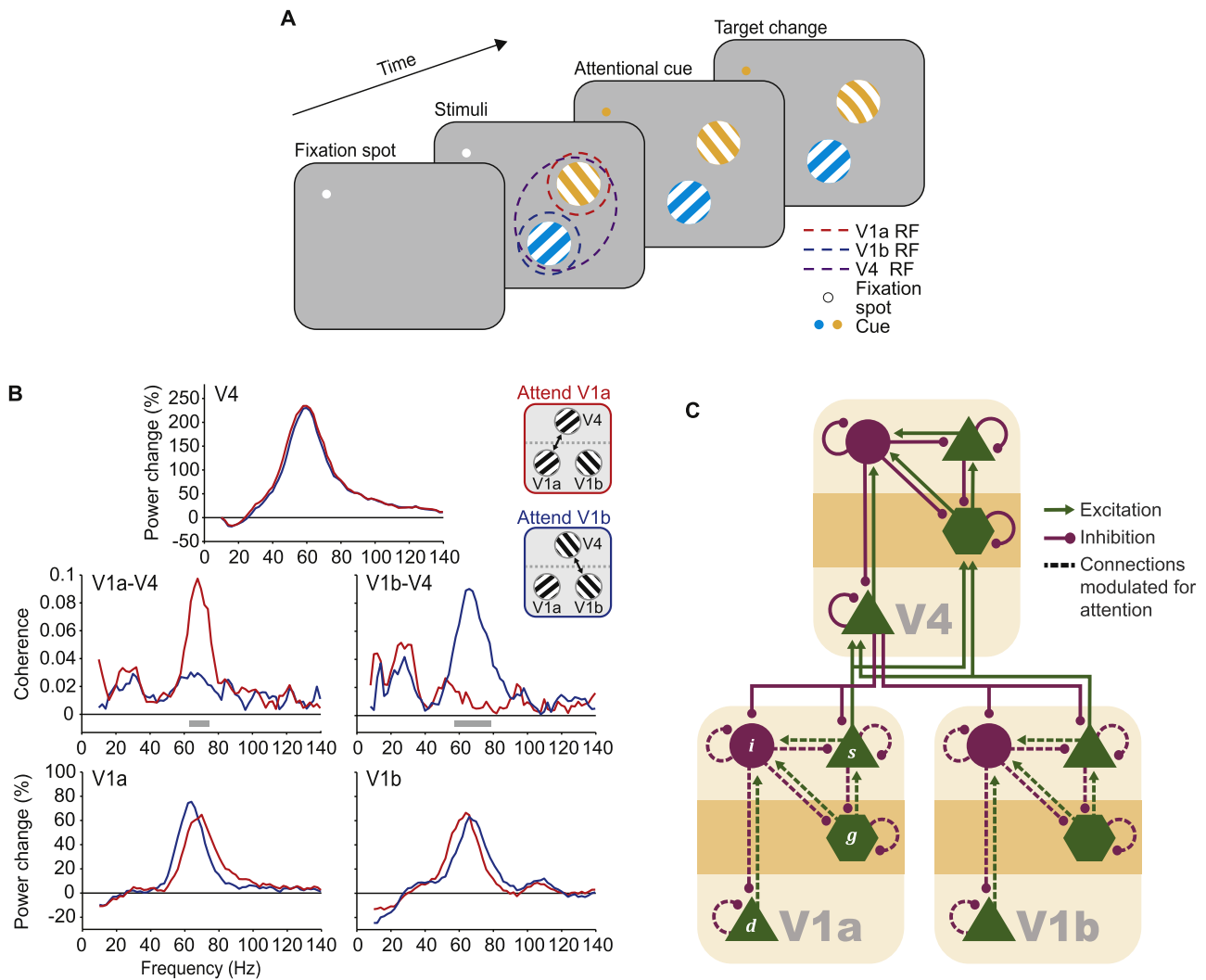
Fig. 1. Modelling the effects of selective attention on gamma-band neuronal synchronization in the visual cortex. (A) Selective attention task (Bosman et al., 2012). The monkey had to maintain fixation on the fixation spot. The stimuli consisted of two iso-luminant gratings, one in the V1a RF, the other in the V1b RF, and both contained in the V4 RF. RFs are illustrated with dashed circles, not visible to the monkey. The color of the fixation spot (cue) indicated which of the two gratings the monkey had to attend. When the cue color matches the color of the stimulus in one V1 RF, the monkey attends that RF location and primarily this attended stimulus is communicated to and represented in the higher area V4. The color assignment to the two stimuli and the attentional condition are selected randomly in each trial. (B) Power and coherence of example V1 and V4 sites from monkey P, while the monkey was instructed to attend the stimulus in the V1a (red lines) or V1b (blue lines) RF. Top : V4 power relative to baseline; bottom : V1 power relative to baseline; middle : V1-V4 coherence spectrum. Modified from Bosman et al. (2012). (C) The V1a-V1b-V4 microcircuit that was used to model the CSD measured from the data. Each area consisted of 4 subpopulations modelled as neural masses: an excitatory population in the granular layer g , a pyramidal population in the supragranular layers s , a pyramidal population in the deep layers d and a population of inhibitory interneurons i . The pattern of intrinsic (within area) and extrinsic (between areas) connectivity is shown. Note that inhibitory (magenta) connections that appear to stem from excitatory (green) populations can be conceived as being mediated by local inhibitory interneurons. Extrinsic connections are depicted as bifurcating to simplify the illustration, but the strength of each of the 8 extrinsic connections was fitted independently. Dashed lines represent the connections whose strength could vary between the two attentional conditions.
