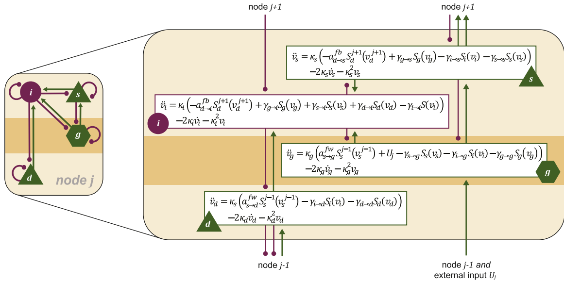
Fig. 2. The canonical microcircuit. Equations of motion for the 4 neural masses within a canonical microcircuit node. v_x , depolarization of population x ; \kappa_x , inverse of time constant of population x ; \alpha_{x \rightarrow y}^{f} , extrinsic feedforward excitatory connection strength from population x to population y ; \alpha_{x \rightarrow y}^{fb} , extrinsic feedback inhibitory connection strength from population x to population y ; \gamma_{x \rightarrow y} , intrinsic excitatory connection strength from population x to population y ; \gamma_{x \rightarrow y} , intrinsic inhibitory connection strength from population x to population y ; S_x , sigmoid function transforming the depolarization of population x to a firing rate; U , external input firing rate; \dot{v} , first temporal derivative of depolarization; \ddot{v} , second temporal derivative of depolarization.
