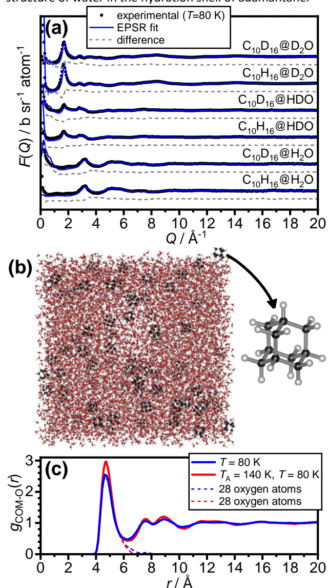
Fig. 2. Fitting of the neutron-diffraction data of the 1:100 adamantane to water samples and the isotropic pair-distribution function of the hydration shells of adamantane. (a) Experimental neutron diffraction data and EPSR fits of the as-made samples at 80 K. (b) Example snapshot of the EPSR simulation and the molecular structure of adamantane ( C_{10}H_{16} ). (c) Pair-distribution function from the centre-of-mass (COM) of adamantane to the oxygen atoms of water for the as-made samples (blue) as well as after annealing at 140 K (red). The contributions from 28 water molecules in the first hydration shell are shown as dashed lines.
