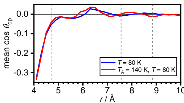
Fig. 5. Net polarisation effects of the hydrophobic hydration. Arithmetic mean of \cos \theta_{\text{dp}} as a function of distance from the COM of adamantane. The maxima in g_{\text{COM-O}}(r) from Fig. 2(c) are shown as grey dashed vertical lines.
