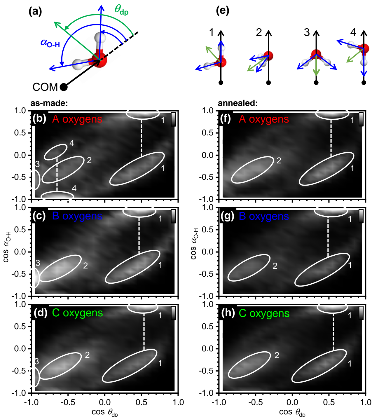
Fig. 4. Orientational ordering of the 28 water molecules in the first hydration shell of adamantane of the as-made samples. (a) Illustration of the angles that define the orientation of the dipole moment of a water molecule, \theta_{dp} , and the direction of an O-H bond, \alpha_{O-H} , within respect to the vector spanning from the centre-of-mass of adamantane to the oxygen atoms of water. (b-d) Orientation-correlation functions of the water molecules with A, B and C type oxygen atoms for the as-made samples. (e) Orientations of the water molecules corresponding to the locations labelled 1-4 in (b-d) and (f-h). (f-h) Orientation-correlation functions of the annealed samples.
