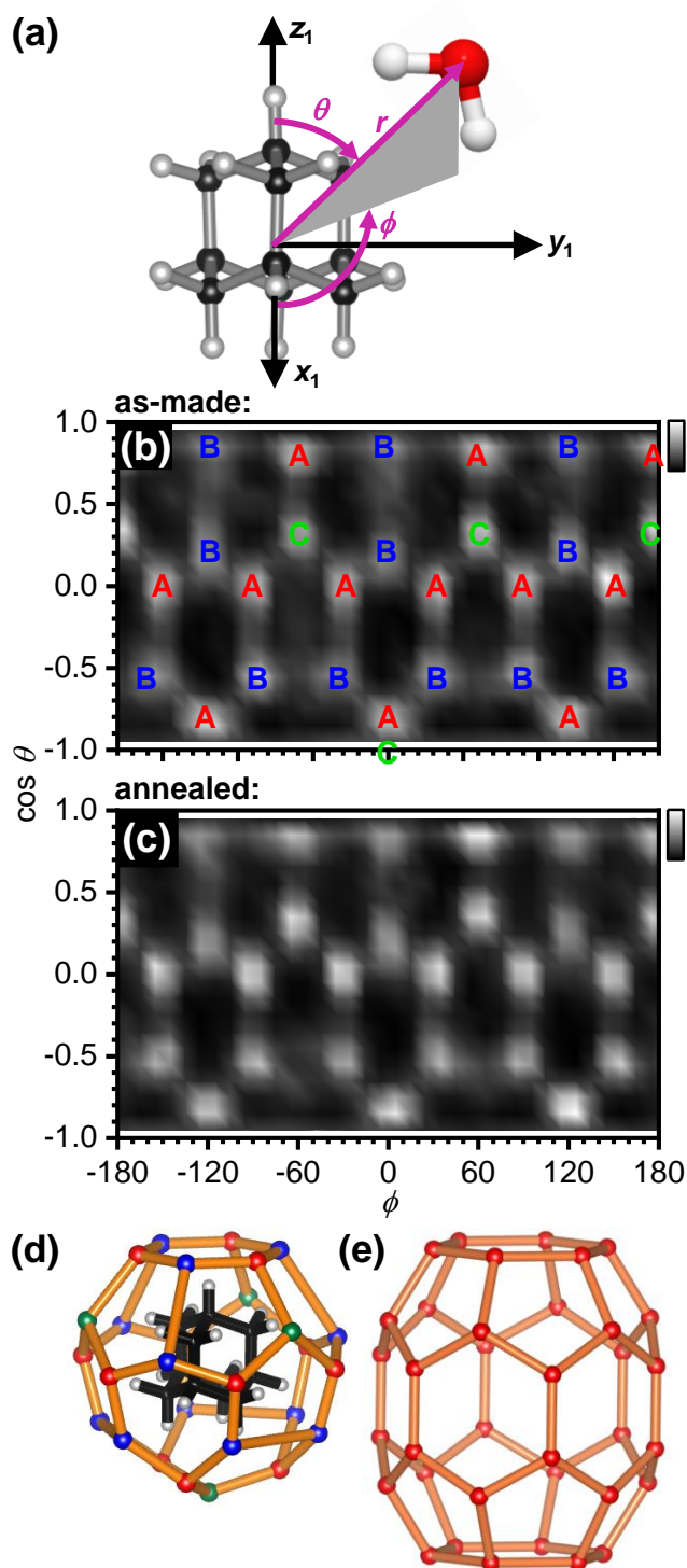
Fig. 3. Structure of the first hydration shell of adamantane. (a) Definition of the spherical
