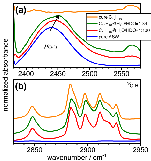
Fig. 6. FT-IR spectra of pure amorphous ice, adamantane matrix-isolated in amorphous ice at 1:100 and 1:34 molar ratios and pure vapour-deposited adamantane in the spectral regions of (a) the decoupled O-D stretching modes 24 and (b) the C-H stretching modes of adamantane. 54 The spectra were shifted vertically for clarity.
