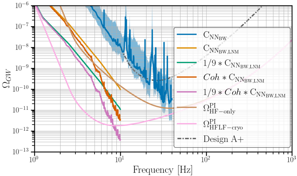
Figure 34. The projected impact from correlated NN from body-waves C_{\text{NNBW}} , as calculated in section III of [141], is shown in blue. The blue line represents the median value, and the associated surface is delimited by the 10% and 90% percentiles. Also curves with more optimistic assumptions (see the text) are shown. Based on figure 16 of [141]. Adapted with permission from [141], copyright (2022) by the American Physical Society.
