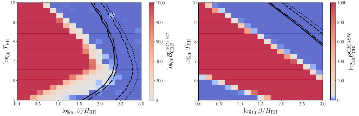
Figure 65. Detectability of bubble collisions (left) and sound wave (right) dominated supercooled FOPT with next-generation ET detector. The dashed line is the detection threshold using 10 km triangular ET configuration, the dotted line is 15 km triangular configuration, while the solid and dot-dashed contours are for two L-shaped detectors with 15 km and 20 km arms, respectively.
