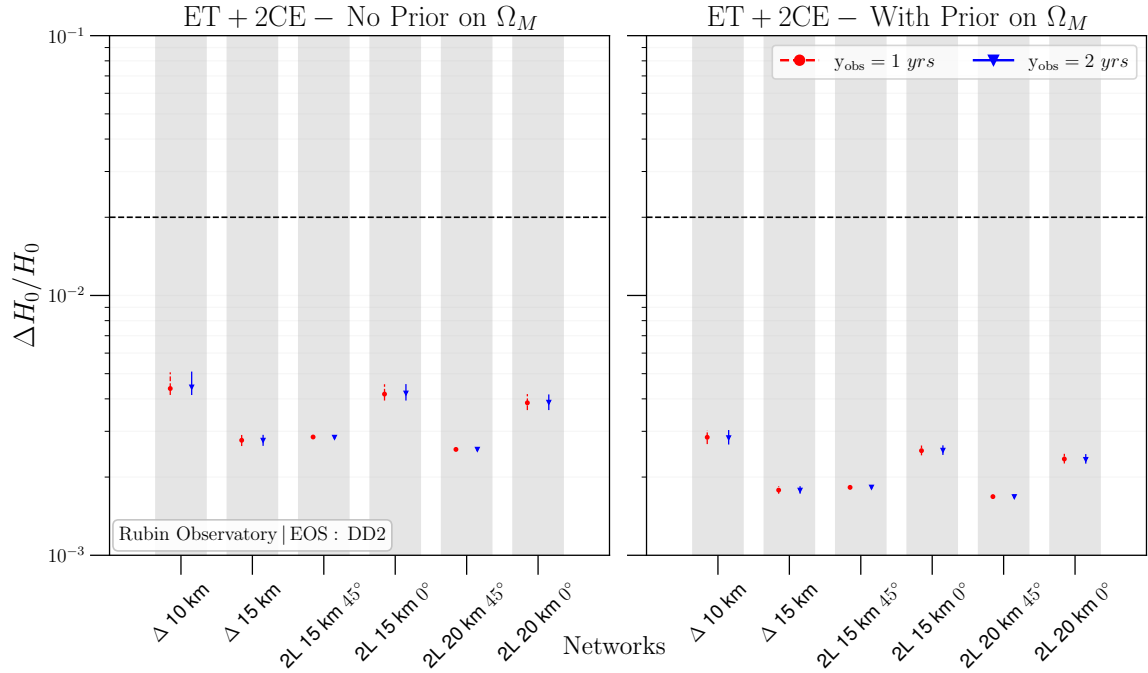
Figure 62. Same as figure 61 except the results are obtained for the NSBH population instead of the BBH population. Moreover, the results were obtained by combining measurement accuracies from systems that produce kilonovae in addition to those that identify a unique host within the localization error box.
