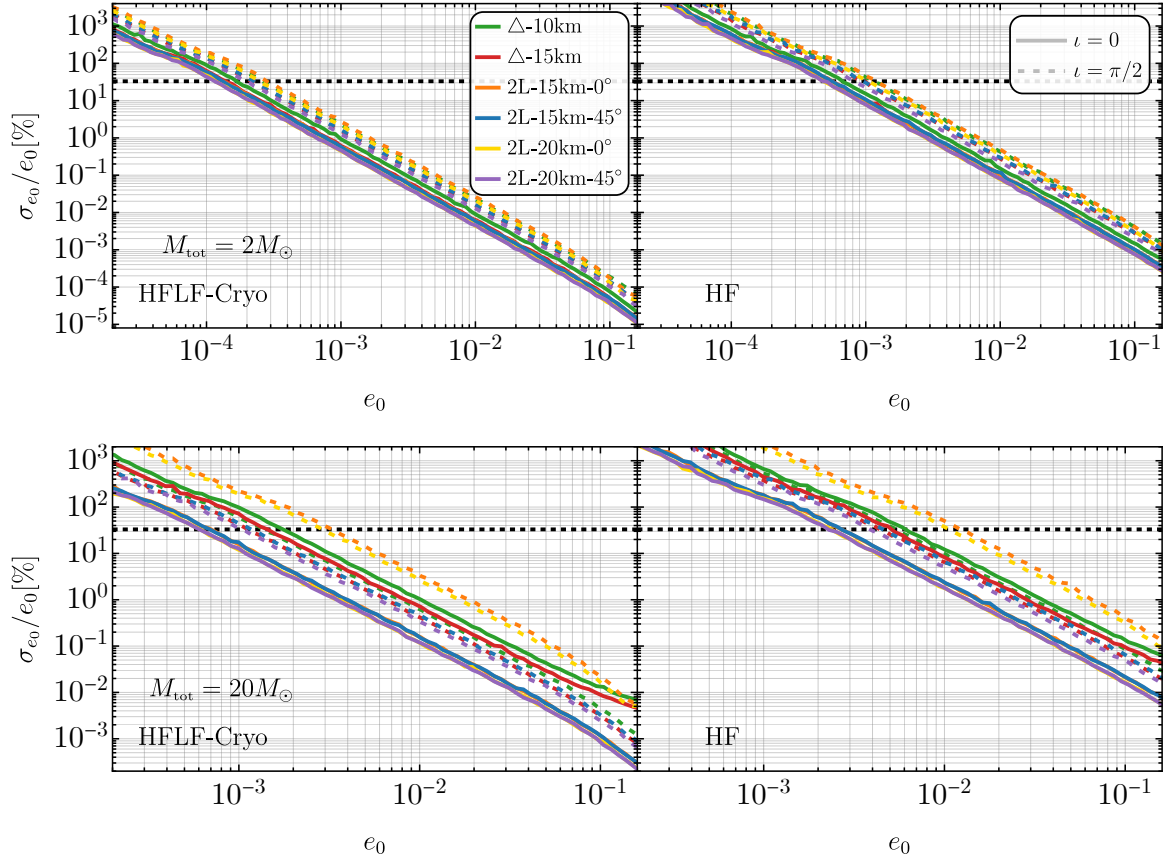
Figure 51. Relative error on the eccentricity e_0 at f_0 = 10\text{Hz} as a function of its injected value for a binary with a total source frame mass of M_{\text{tot}} = 2M_\odot and d_L = 100\text{ Mpc} in the upper panel, while M_{\text{tot}} = 20M_\odot and d_L = 500\text{ Mpc} in the lower panel. For the range of eccentricities in the horizontal axis (that are too large for PBH binaries), one is able to exclude (at 3\sigma level) a PBH origin for events that fall below the horizontal black dashed line.
