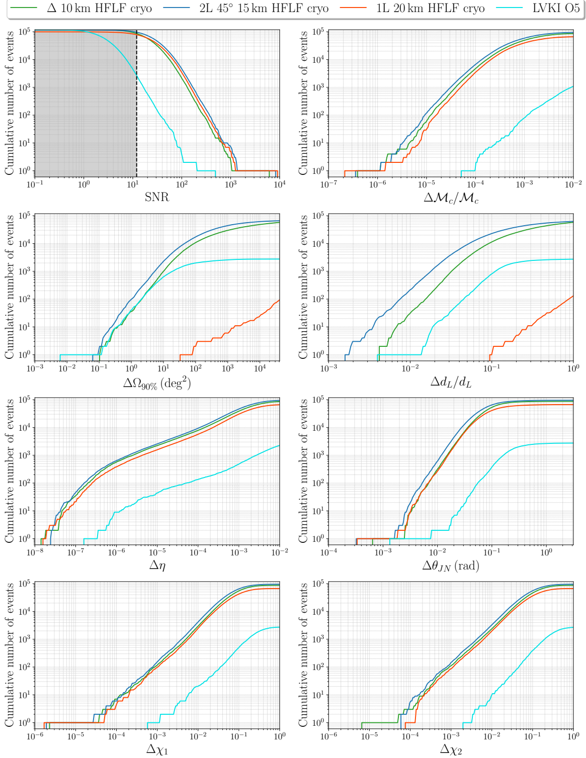
Figure 7. Comparison of SNR and parameter estimation error for the 10 km triangle, 15 km L misaligned and a single 20 km L with the HFLF-cryo ASD. By comparison, we also show the forecast for LVKI O5.
