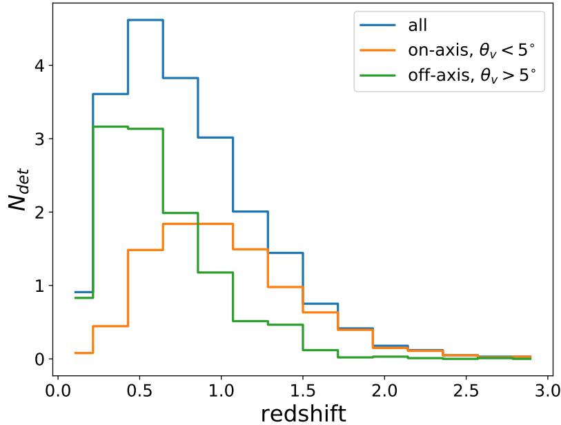
Figure 25. Redshift distribution of joint GW+EM detections with THESEUS-(SXI+XGIS) in survey mode, where we distinguish between on-axis and off-axis cases. The ET configuration considered here is 2L 20 km HFLF cryo.
