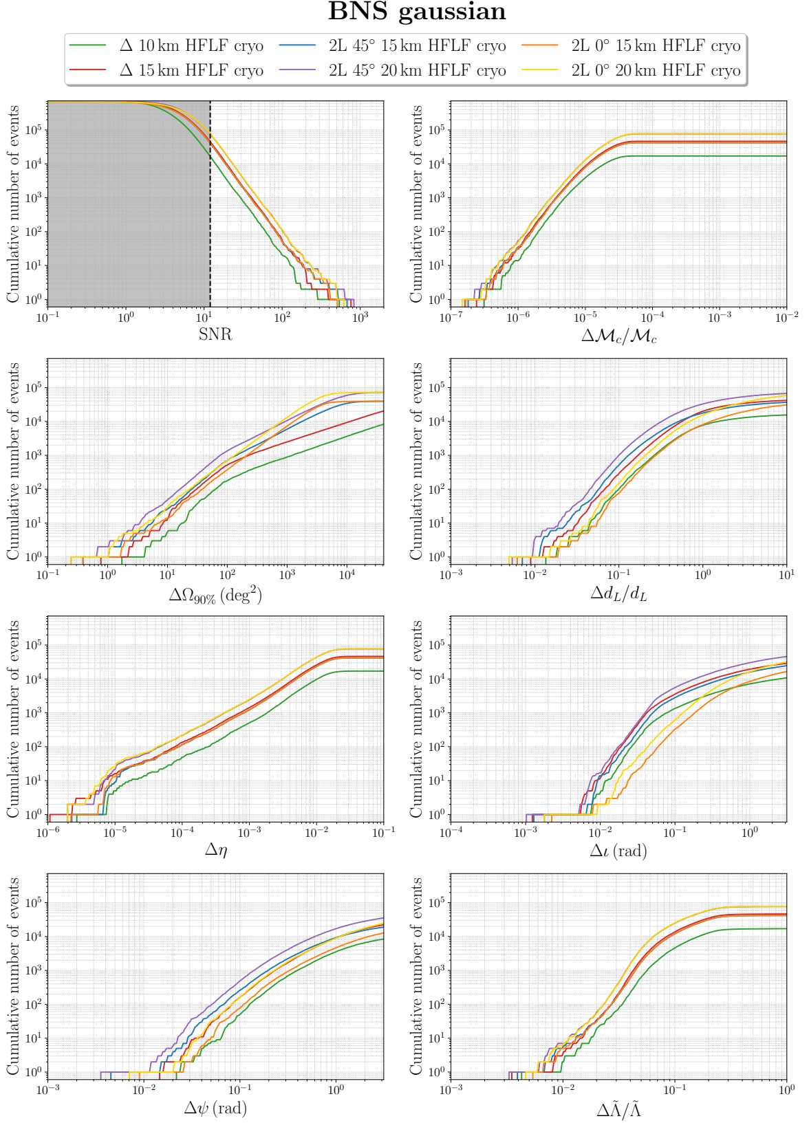
Figure 17. As in figure 11, for a gaussian mass distribution of the two component neutron stars.
