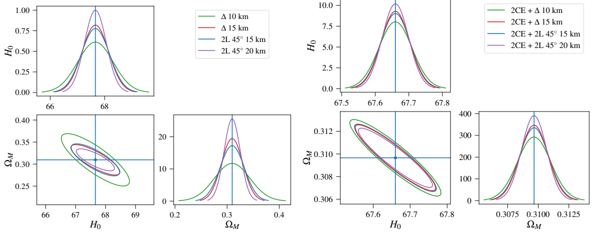
Figure 58. Constraints on the parameters H_0 and \Omega_M in \Lambda CDM model using one year GW observations from BNS alone for different ET geometries. The covariance for a standalone ET is shown in the left panel while ET in a network with 2CE is shown in the right panel. H_0 is measured in \text{km s}^{-1} \text{Mpc}^{-1} .
