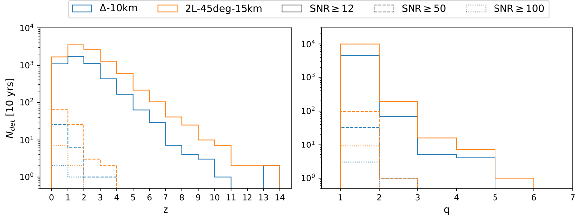
Figure 37. Ringdown event rates as a function of redshift (left) and mass ratio (right) for the baseline 10km triangle and the 15km-45°-2L configuration. Different colors indicate detectors configurations; continuous, dashed, and dotted contours indicate different ringdown SNR thresholds.
