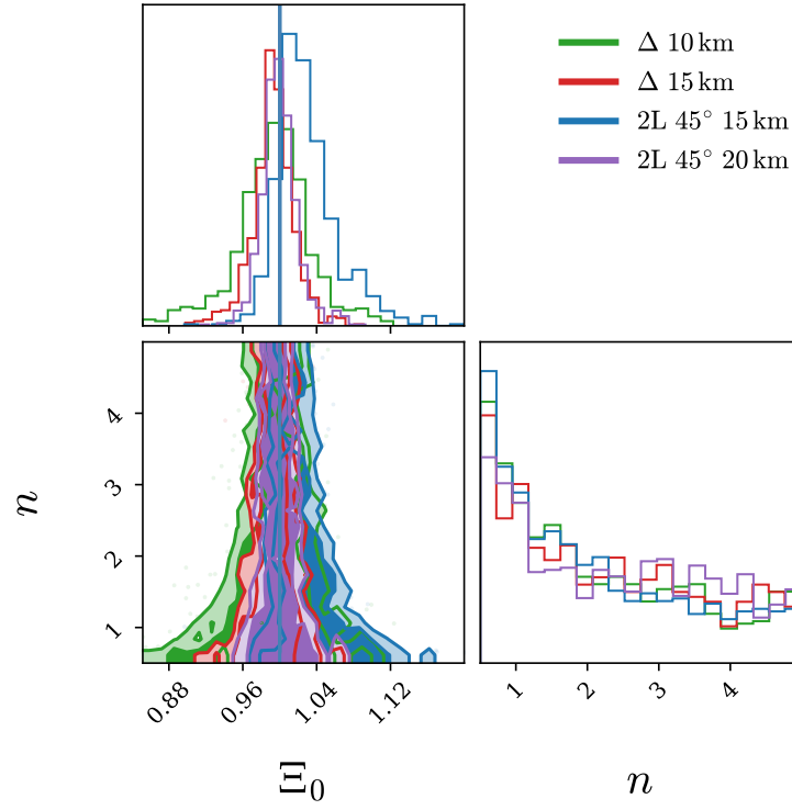
Figure 56. Reconstruction of the parameters \Xi_0 and n in modified gravity, from the joint GW+EM events obtained with ET+THESEUS in 5 yr of observations, for the different geometries of ET shown, all with their HFLF-cryo sensitivity.
