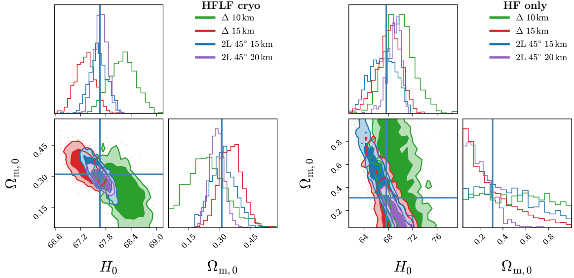
Figure 53. Reconstruction of the parameters H_0 and \Omega_M in \Lambda CDM, from the joint GW+EM events obtained with ET+VRO in 1 yr of observations, for the different geometries of ET shown, in the left panel with their HFLF-cryo sensitivity and in the right panel with the HF instrument only.
