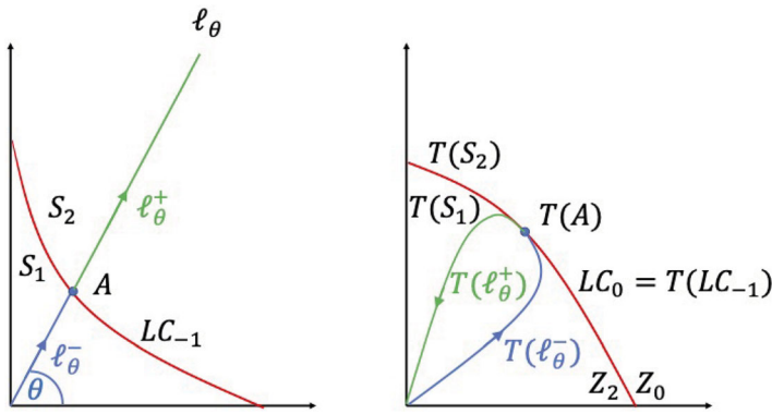
Figure A1. T maps the line \ell_{\theta} onto a simple curve T(\ell_{\theta}) = T(\ell_{\theta}^{+}) \cup T(\ell_{\theta}^{-}) and \overline{T(\ell_{\theta})} is a closed curve joining O to itself. T maps S_1 onto T(S_1) and S_2 onto T(S_2) where T(S_1) = T(S_2) \cup \{O\} . The envelope of all curves T(\ell_{\theta}) is LC_0 = T(LC_{-1}) . C_+ = Z_2 \cup LC_0 \cup Z_0 where points in Z_0 have no preimage, and points in Z_2 have 2 preimages. That the curve T(\ell_{\theta}) encloses a convex set can be shown fairly easily by showing that the curvature of T(\ell_{\theta}) does not vanish.
