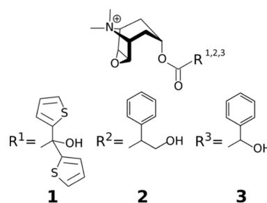
Figure 1. Structures of the ligands investigated in this study: tiotropium (1), N -methylscopolamin (2), and homatropine methylbromide (3).
