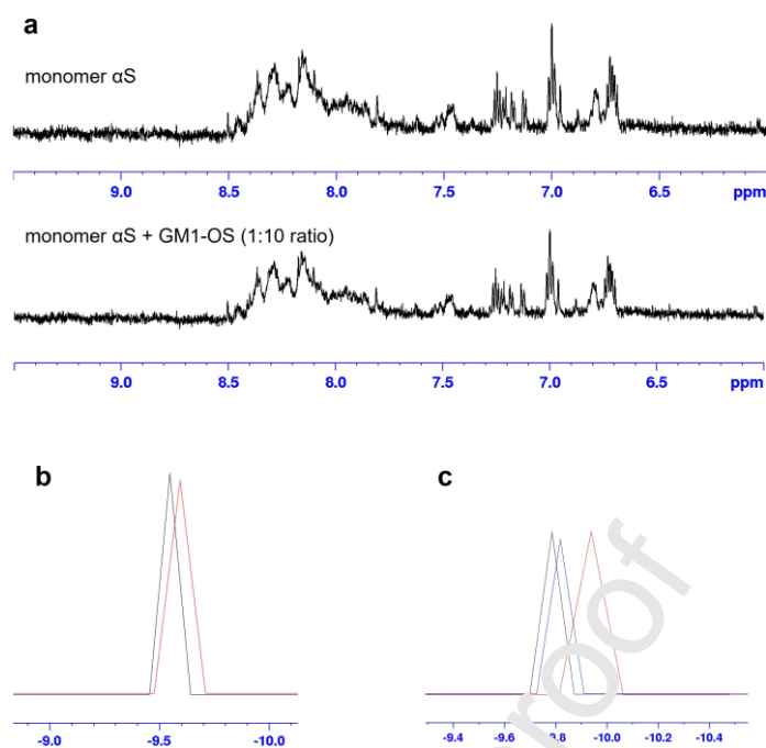
Figure 5. NMR interaction studies between GM1-OS and \alpha S. (a) 1D NMR region of the backbone NHs of \alpha S alone (top) and \alpha S in presence of GM1-OS (bottom): the two regions show the same spread of NHs chemical shift, suggesting that no changes in the secondary structure occurs; (b) logD values calculated for GM1-OS alone (black) and after the addition of \alpha S in a 10:1 ratio (red): the diffusion coefficient is slightly decreased indicating the presence of an equilibrium with a bound form to \alpha S; (c) logD values obtained for \alpha S alone (black), \alpha S alone after 60 h (red) indicating a spontaneous aggregation process and \alpha S in presence of GM1-OS after 60 h (blue) where no aggregation phenomena can be observed.
