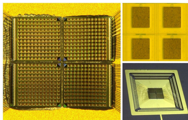
Figure 24. Left: Photo of a THz camera based on 150 nm CMOS technology (LFoundry). The detectors have a room temperature sensitivity of approximately 300 \text{ V W}^{-1} and noise equivalent power (NEP) of 43 \text{ pW } (\sqrt{\text{Hz}})^{-1} at 600 GHz with full width at half maximum (FWHM) of 62 GHz. Pitch separation between pixels is 195 \mu\text{m} . Pixel number—568. Right: Enlarged pixel elements (top) and overall view of the focal plane array bonded to a chip holder (bottom). Courtesy of the Frankfurt/M group.
