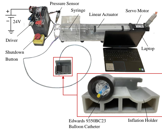
Fig. 1. Experimental setup for sizing and measuring idealised aortic annular compliant phantoms.
