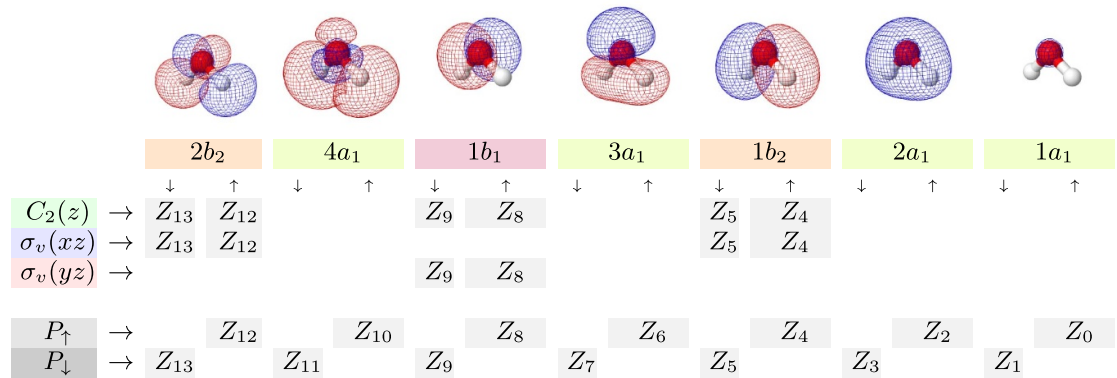
Figure 5. In the Jordan–Wigner encoding, where each qubit corresponds to a spin-orbital given by the symmetry-adapted linear combinations of molecular orbitals, the qubit operators corresponding to Boolean symmetries have a particularly simple form. We see that the three non-identity elements of the point-group C_{2v} are mapped to a (tensor) product of Pauli Z operators acting on the orbitals that are antisymmetric with respect to them, using the information contained in the point-group character table that was given in figure 3. It is easy to see that the group operation is respected by the mapping, as for example the product of symmetry operators C_2(z) \times \sigma_v(xz) = \sigma_v(yz) is mirrored by the product of qubit operators Z_{13}Z_{12}Z_9Z_8Z_5Z_4 \times Z_{13}Z_{12}Z_5Z_4 = Z_9Z_8 . Finally, the two parity operators P_\uparrow and P_\downarrow are mapped to Pauli Z operators on those qubits that correspond to spin-up and spin-down spin-orbitals respectively.
