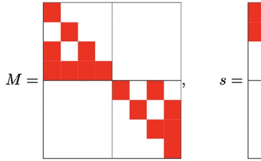
Figure 6. The Clifford tableau for the example given by equation (12), where red squares correspond to a matrix element equal to 1 and white squares to 0, and the columns (rows) of the matrix M correspond to the Pauli operators Z_0, Z_1, Z_2, Z_3, X_0, X_1, X_2, X_3 from left to right (from top to bottom). The corresponding Clifford operator followed by a projection maps qubit operators in the Jordan–Wigner encoding to the corresponding symmetry-adapted encoding qubit operators, for the example of the ground state eigensector of H_2 on a minimal basis.
