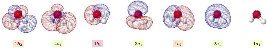
Figure 4. Isosurfaces for the molecular orbitals of the water molecule ( \text{H}_2\text{O} ) in a minimal basis constructed as symmetry-adapted linear combinations of atomic orbitals, in order of ascending energy starting from the right (this follows the convention that will be used for the rest of the article). The orbitals are named by the irreducible point group ( C_{2v} ) representation they lie in (in this case A_1 , B_1 and B_2 ). Of the 2^{14} = 16\,384 possible Slater determinants that can be formed from the molecular orbitals, exactly 2^{12} = 4096 lie in each of the four irreducible representations: for instance the four computational states corresponding to the configuration 2b_2 1b_1 3a_1 1b_2 2a_1^2 1a_1^2 all lie in the A_2 irreducible representation. Each of the seven molecular orbitals corresponds to two spin-orbitals, each of which in turn corresponds to a qubit in the JW encoding, for a total of 14 qubits. In the symmetry-adapted encoding for the water molecule this number is reduced to 10 qubits.
