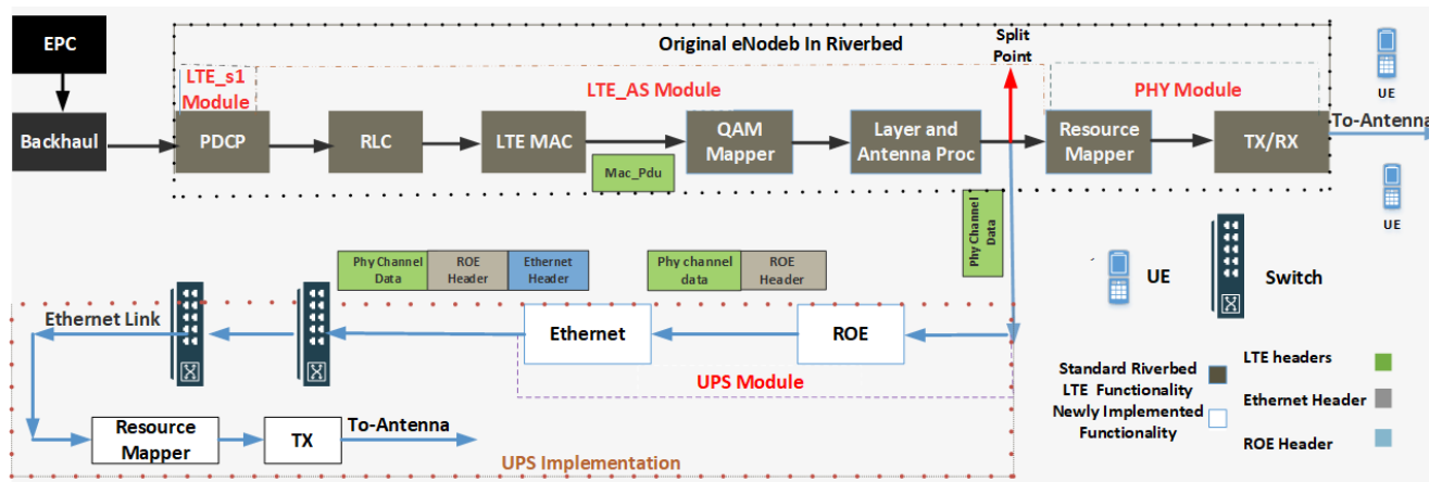
Fig. 1. Implementation of the UPS in the Ethernet fronthaul network. EPC, Evolved Packet Core; LTE_AS, LTE Access Stratum; Tx/Rx, Transmit/Receive; RoE, Radio-over-Ethernet; UE, User Equipment; PHY, Physical layer; PDU, Protocol Data Unit; QAM, Quadrature Amplitude Modulation.
