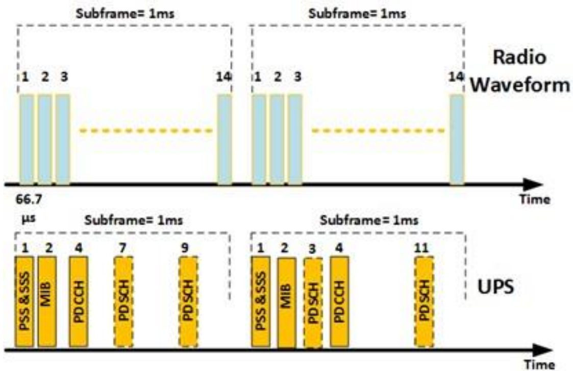
Fig. 2. UPS and Radio Waveform traffic transmission pattern,
