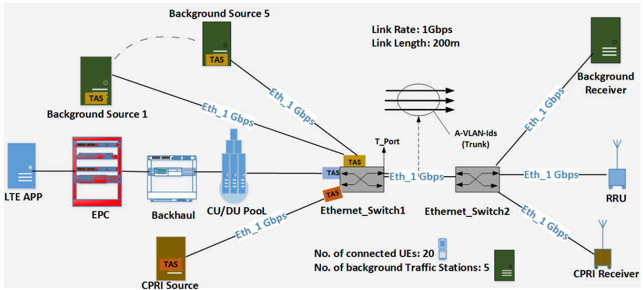
Fig. 3. The simulation set-up of the Ethernet fronthaul.
