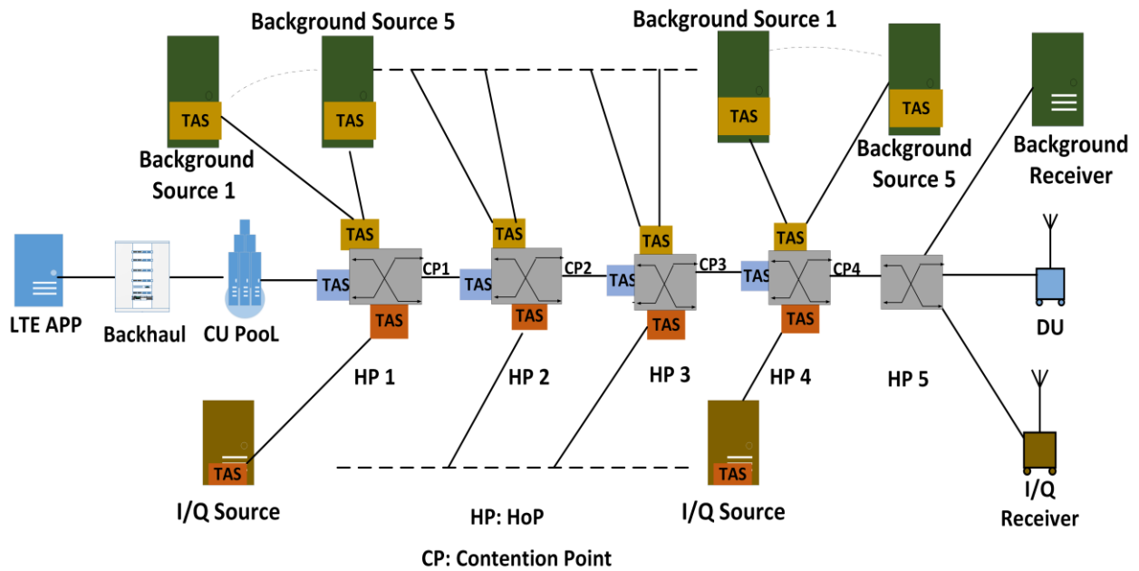
Fig.11. Ethernet fronthaul with TAS and five hops.
