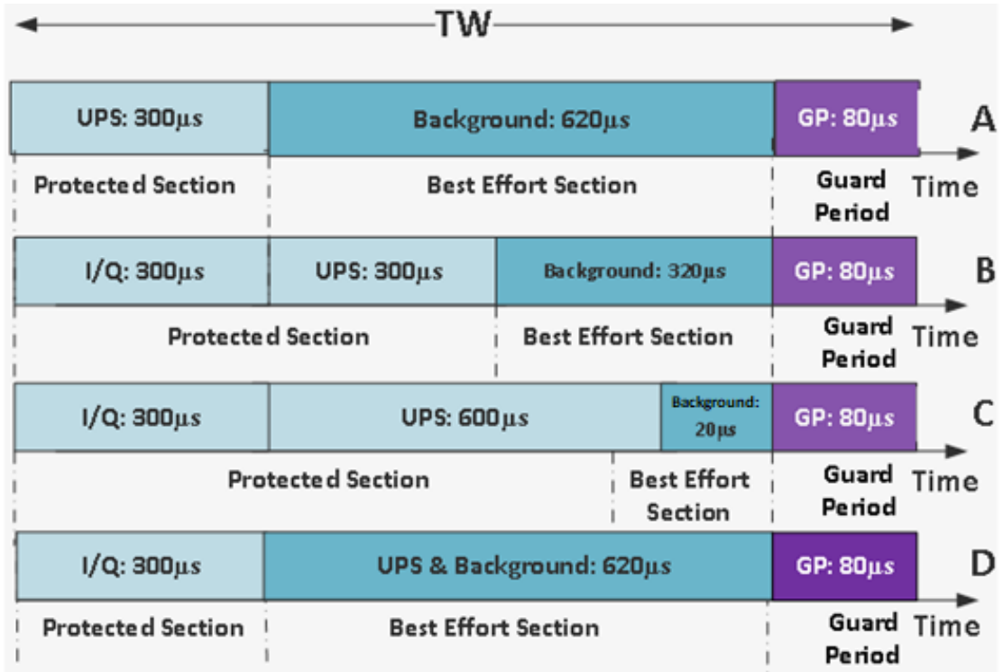
Fig. 7. TAS section allocations in: (A) UPS and background traffic scenario; (B) Mixed traffic scenario (case 1); (C) Mixed traffic scenario (case 2); (D) Mixed traffic scenario (case 3).
