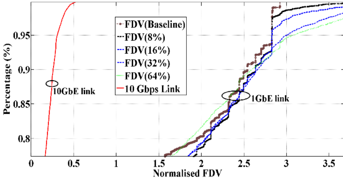
Fig. 10.A. CDF of the UPS FDV for different link utilizations.
