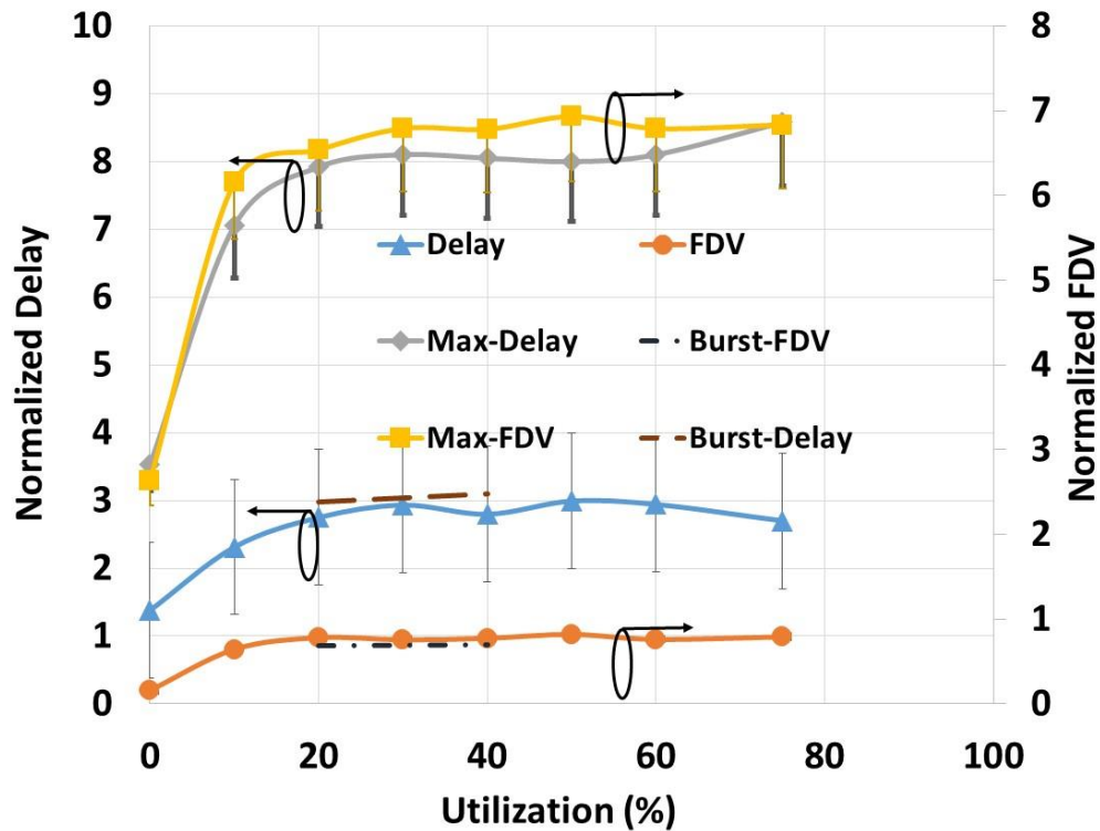
Fig. 5. UPS traffic delay and FDV for different background traffic data rates (scenario B). Special case of delay and FDV with bursty background traffic is presented.
