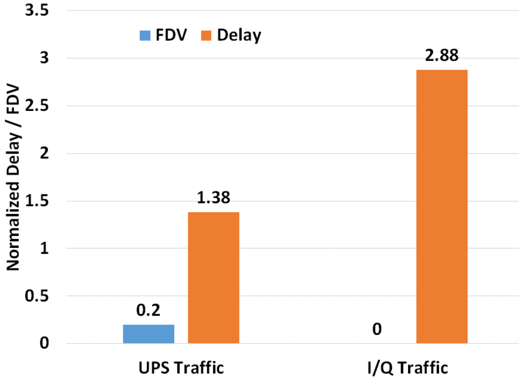
Fig. 4. Baseline delay and frame delay variation (FDV) of the UPS and I/Q-type traffic.
