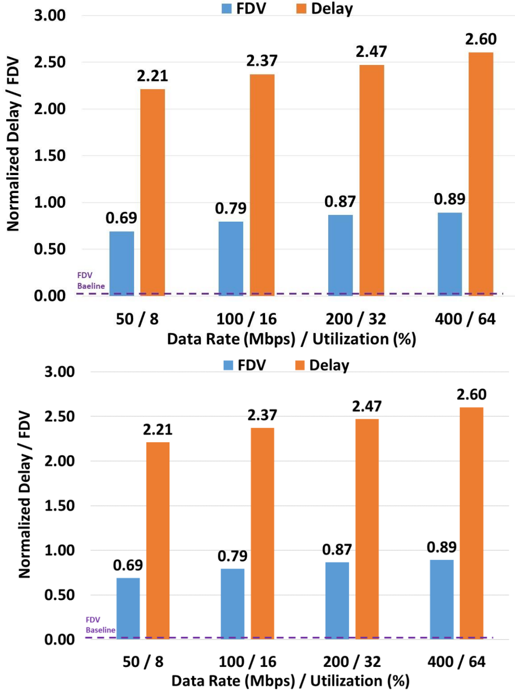
Fig. 9. Frame delay and FDV of UPS traffic with TAS when UPS is allocated to the BES for different background traffic data rates (scenario C). The traffic percentage corresponds to different utilizations of the BES window.
