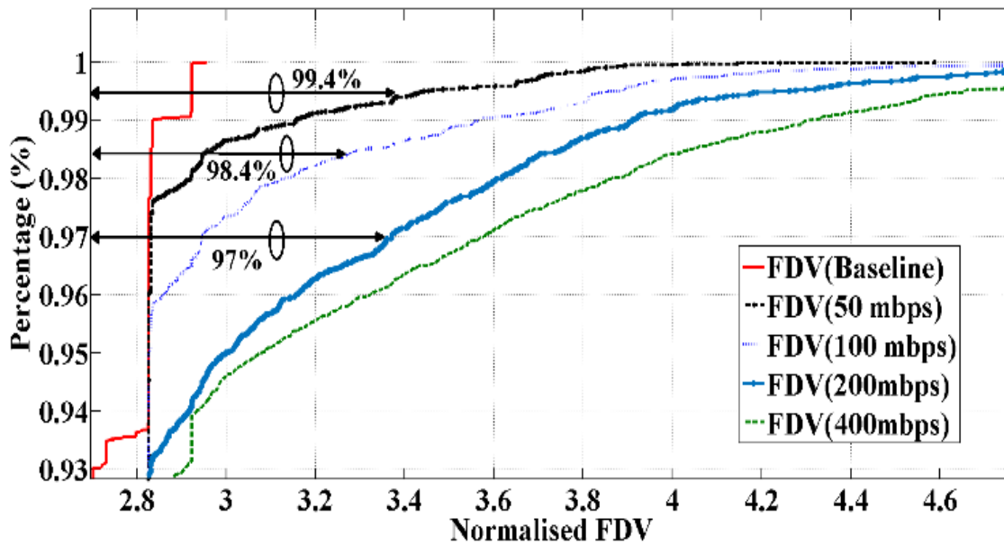
Fig. 10.B. Zoomed UPS FDV's CDF result.
