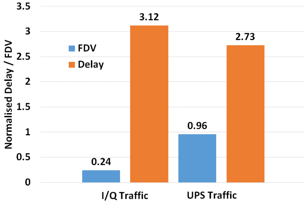
Fig. 6. UPS & I/Q traffic delay and FDV with the existence of background traffic (scenario C).
