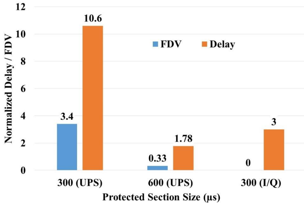
Fig. 8. Frame delay and FDV of I/Q-type and UPS traffic with TAS, for different window section allocations for the UPS traffic (300 µs and 600 µs) (scenario B).
