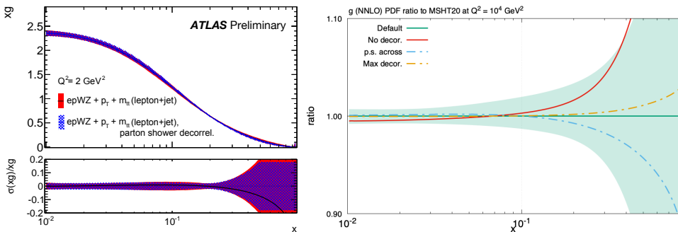
Fig. 11. Left: difference in the gluon PDF shown in ratio to the ATLASepWZtop18 gluon (called \text{epWZ}+p_T^t+m_{tt} ). The use of full correlation of all systematic sources (red) is compared to the result when decorrelating the parton shower systematic between the p_T^t and m_{tt} spectra (blue). Right: differences between the scenarios with the default systematic error treatment, no decorrelation, decorrelation only across distributions, and full decorrelation for the gluon PDF from [9].
