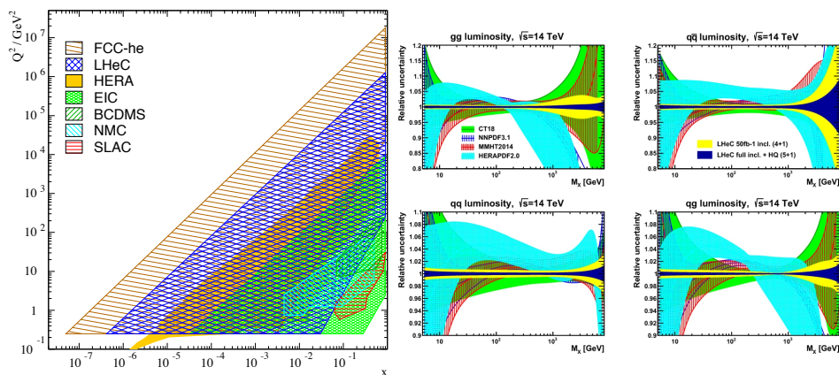
Fig. 9. Left: Coverage of the kinematic plane in deep inelastic lepton-proton scattering by some initial fixed target experiments (SLAC, NMC, BCDMS), and by the ep colliders: the EIC (green), HERA (yellow), the LHeC (blue), and the FCC-he (brown). Figure from Ref. [30]. Right: Expected precision for the parton-parton luminosities as a function of M_X in Drell-Yan scattering at the LHC at \sqrt{s} = 14 TeV for three recent PDFs (shaded areas) and for PDFs from LHeC (full areas) shown for an initial 3-year LHeC run (yellow) and the full LHeC data set (dark blue). Figure from Ref. [155].
