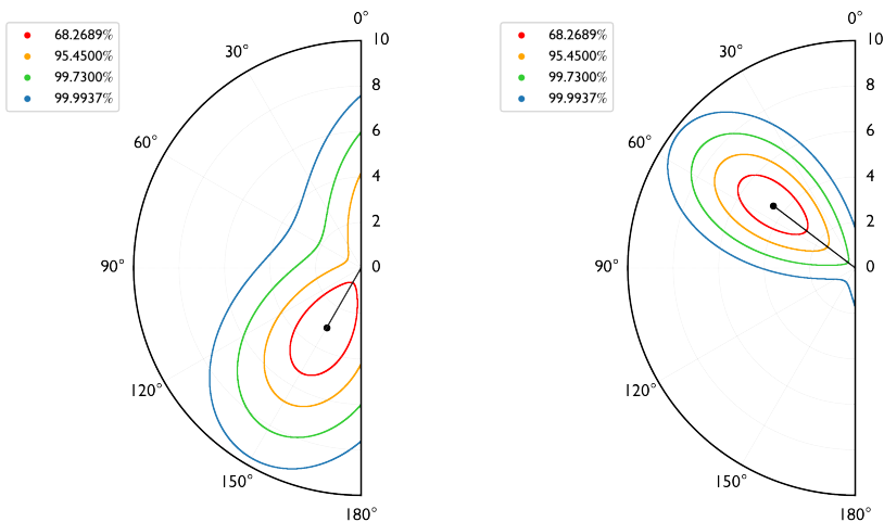
Fig. 7 Polar plot of the \Pi_x - \psi_x plane. Confidence contours of X-ray polarization derived within ixpeobssim for IXPE are shown for Obs. 2 (left panel) and 3 (right panel) of Mrk 421. The polarization degree is displayed in percentage units. For each case, the contours at 68.26%, 95.45%, 99.73%, and 99.994% confidence level (considering two degrees of freedom) are displayed, colour-coded in red, yellow, green, blue.
