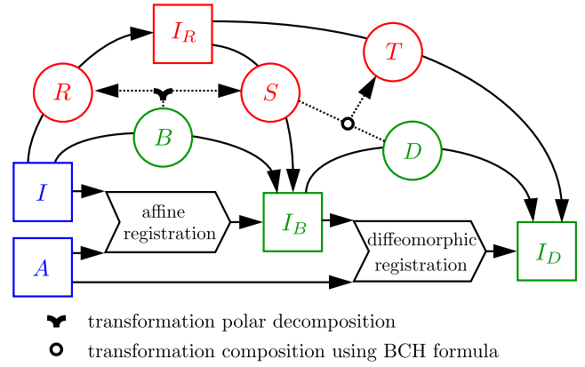
Fig. 2. Illustration of the registrations and operations on transformations. Squares design images whereas circles represent transformations. In blue the initial images ( I new subject and A current atlas), in green the outputs of the registrations ( B terms for affine, and D for diffeomorphic), and in red the components extracted from the operations on the registration transformations.
