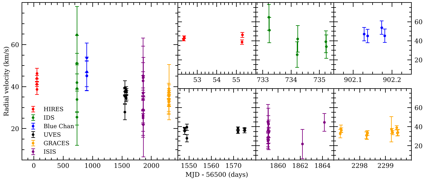
Figure 4. All radial velocities and their errors for PG 0010 + 281 as determined from H\alpha line fitting. The six panels on the right show zoomed-in regions of the left-hand panel. The observations span just over 6 years, and have been acquired with six different instruments, each designated in the plot legend with a distinct symbol colour (see Table 1). Measurements are plotted as a function of MJD both for the overall, multi-instruments data set, as well as for individual instruments. The plotted data are uncorrected for any systematic offsets between instruments.
