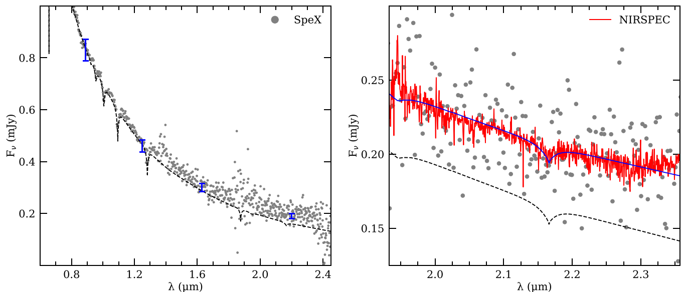
Figure 7. Infrared spectra of PG 0010 + 281. The left-hand panel shows the SpeX prism spectrum (grey points), together with the same photometry (blue error bars) and white dwarf atmospheric model (black dashed line), as shown in Fig. 8. The right-hand panel shows the NIRSPEC spectrum in red, offset to match the K -band photometric flux, and with a weak but clear detection of \text{Br}\gamma from the stellar photosphere. The SpeX data and the white dwarf model atmosphere are also plotted as on the left, where the blue solid line includes the addition of a 1000 K blackbody. The upturn near 2.3\ \mu\text{m} in the NIRSPEC data are not seen in the SpeX data, and thus may be an artefact of the reduction process or instrument settings.
