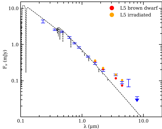
Figure 8. The photometric spectral energy distribution of PG 0010 + 281. Blue error bars show GALEX near-ultraviolet, optical SDSS ugriz , and Spitzer IRAC fluxes (measured here independently). The stellar photosphere is plotted as a black-dashed line, and modelled using a 27 000 K pure hydrogen atmosphere white dwarf (Koester 2010). Also plotted are models that include the addition of flux from an L5-type brown dwarf, both without (red circles) and with (orange circles) the influence of stellar irradiation. The brown dwarf fluxes are derived from an extensive study of M, L, and T dwarfs using Spitzer IRAC (Patten et al. 2006), and the effects of irradiation were estimated based on the observed IRAC variability for WD 0137–349 (Casewell et al. 2015). The IRAC 3.6 \mu\text{m} and 4.5 \mu\text{m} data for PG 0010 + 281 were 10–15 min apart, where an irradiated companion could change aspect somewhat for relatively short orbital periods.
