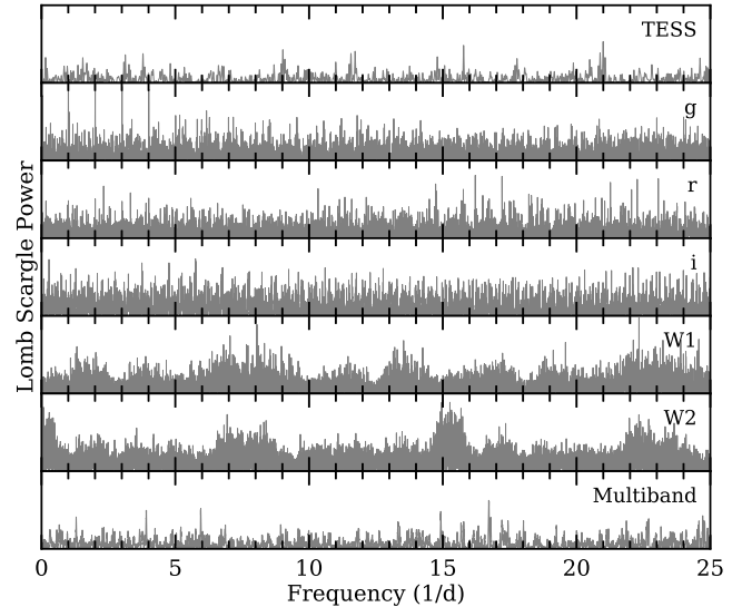
Figure 6. LS periodograms for PG 0010 + 281 photometry. From top to bottom, the panels correspond to: TESS , ZTF gri , WISE W1 and W2, and a multiband periodogram that combines all of the aforementioned photometry. There are no significant periods except at aliases expected from ground-based observations, where the top of the y-axis range corresponds to a 1 per cent false alarm probability level in each panel.
