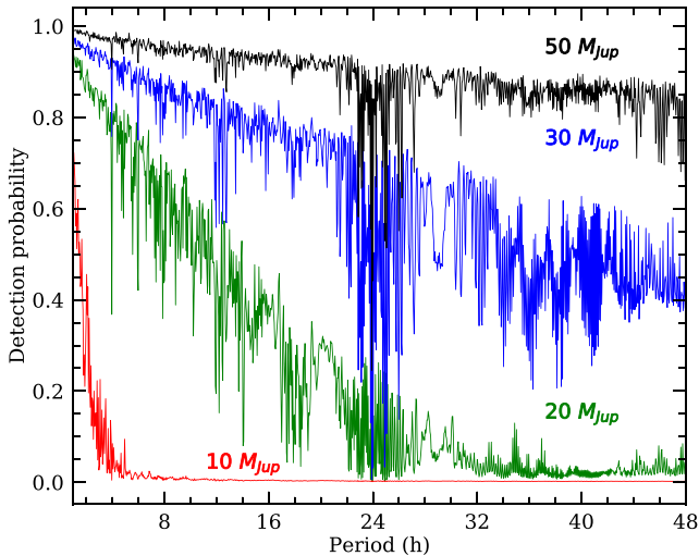
Figure 5. Detection probabilities as a function of orbital period for a range of substellar companion masses, based on a \chi^2 test and the combined radial velocity data from IDS, UVES, ISIS, and GRACES. Of particular interest is the region below 12 h, which spans the orbital periods of all known white dwarf – brown dwarf binaries (Zorotovic & Schreiber 2022). These brown dwarf companions to white dwarfs have masses in the range 50–70 M_{\text{Jup}} , for which the detection probabilities are typically above 0.9.
