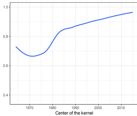
C. Clustering
