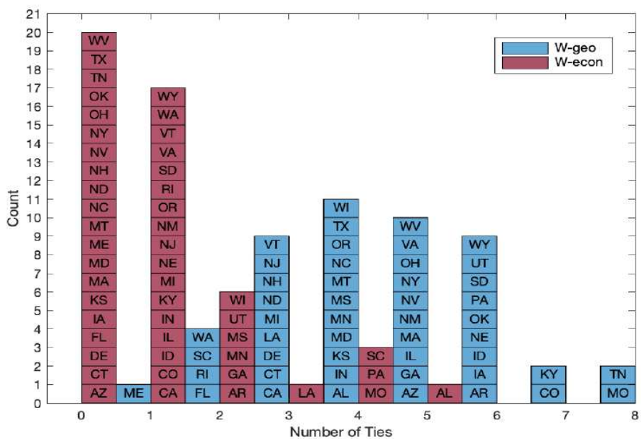
Figure 2: Out-degree Distribution
