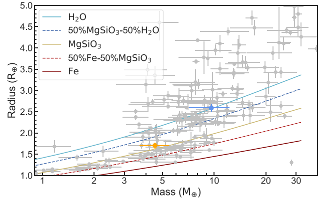
Figure 13. Mass-radius diagram plotted for TOI-836 b in orange and TOI-836 c with exoplanets from the TEPICAT catalogue (Southworth 2011) in grey and composition models from Zeng, Sasselov & Jacobsen (2016).
