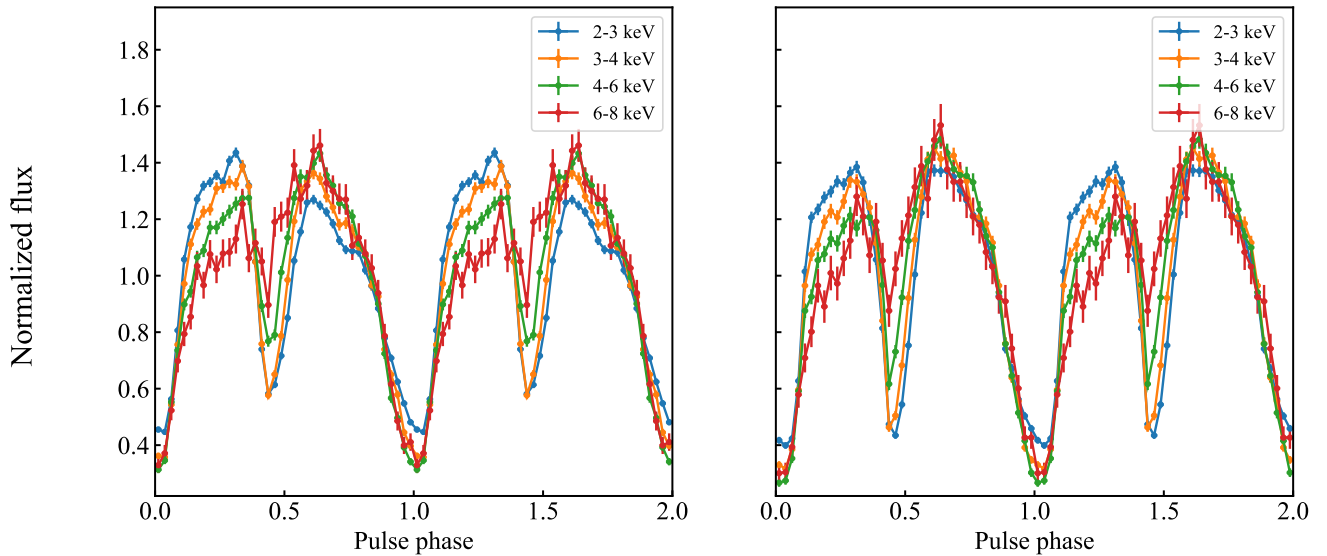
Fig. 2. Pulse profile of GRO J1008–57 in different energy bands as seen by IXPE in the bright (left) and low (right) states. Data from the three telescopes were combined. The zero phase was chosen to coincide for both observations using cross-correlation of the profiles.
