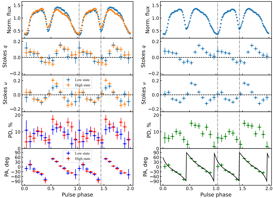
Fig. 4. Dependence of the normalized flux in the 2–8 keV energy band, normalized Stokes parameters q and u (based on the formalism by Kislak et al. 2015), PD, and PA (from the spectro-polarimetric analysis) on the pulse phase for two IXPE observations separately (left) and combined (right). Data from the three IXPE telescopes are combined. Vertical dash-dotted lines show the positions of two minima in the profile and are added for illustrative purposes. The black solid line in the bottom right panel shows the best-fit rotating vector model (see Sect. 4.2).
