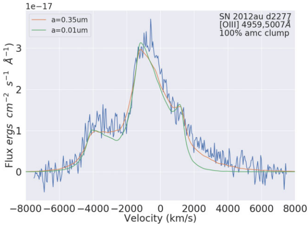
Figure 24. The best-fitting model for SN 2012au’s day 2277 [O III] 4959, 5007 Å doublet feature, using a clumped amorphous carbon dust distribution with a grain radius of 0.35 \mu\text{m} and a dust mass of 4 \times 10^{-4} M_{\odot} , with the other parameters described in Table 8. This can be seen to provide a better fit to the observed profile than the best-fitting model using clumped amorphous carbon dust with a smaller grain radius of 0.01 \mu\text{m} and a dust mass of 1 \times 10^{-4} M_{\odot} , with otherwise matching model parameters.
