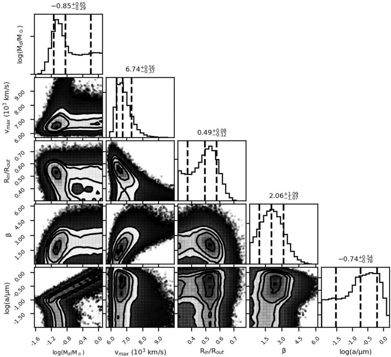
Figure A3. The full posterior probability distribution for the 5D model of SN 1979C's [O II] 7319, 7330 Å profile at day 13 903, using 100 per cent carbon dust. The contours of the 2D distributions represent 0.5\sigma , 1.0\sigma , 1.5\sigma , and 2.0\sigma and the dashed, black vertical lines represent the 16th, 50th, and 84th quantiles for the 1D marginalized probability distributions.
