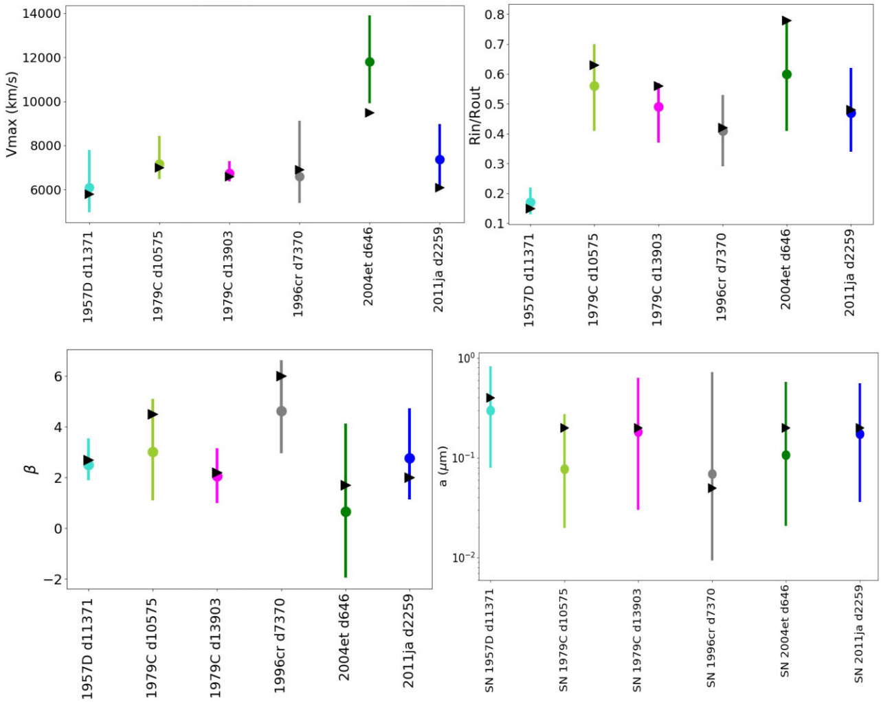
Figure A8. The V_{\max} , R_{in}/R_{out} , \beta , and \log(a) parameters derived from manual fits (black arrowheads), and the median values (circles) of the same parameters taken from the 1D posterior distribution from Bayesian models, with the 16th and 84th quartile of the distribution as the uncertainty limits, for a range of CCSNe studied in this work.
