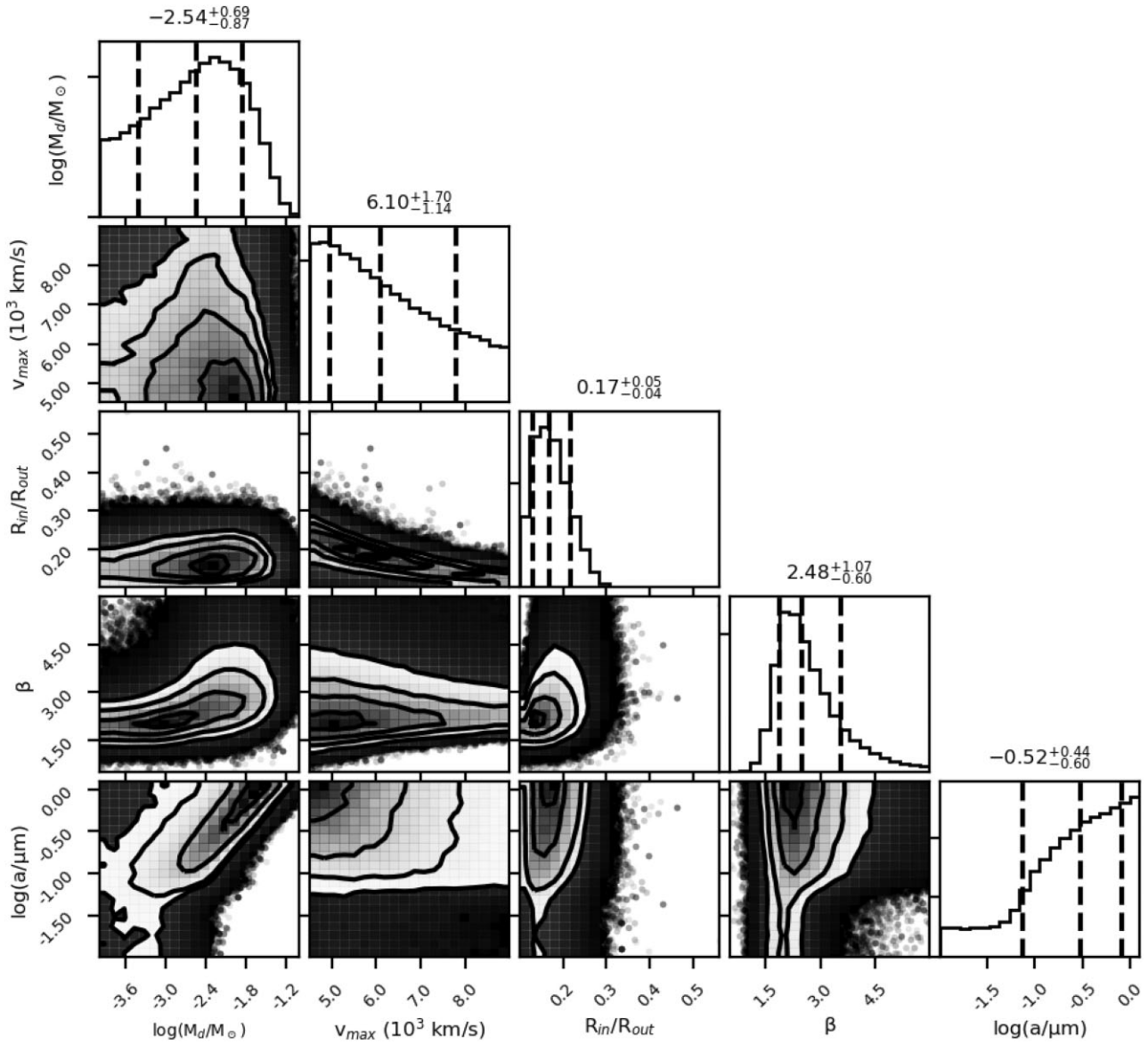
Figure A1. The full posterior probability distribution for the 5D model of SN 1957D's [O III] profile at day 11 371, using 100 per cent carbon dust. The contours of the 2D distributions represent 0.5\sigma , 1.0\sigma , 1.5\sigma , and 2.0\sigma and the dashed, black vertical lines represent the 16th, 50th, and 84th quantiles for the 1D marginalized probability distributions.
