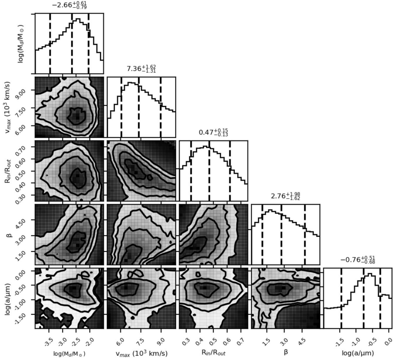
Figure A6. The full posterior probability distribution for the 5D model of SN 2011ja's H \alpha profile at day 2259, using 100 per cent silicate dust. The contours of the 2D distributions represent 0.5\sigma , 1.0\sigma , 1.5\sigma , and 2.0\sigma and the dashed, black vertical lines represent the 16th, 50th, and 84th quantiles for the 1D marginalized probability distributions.
