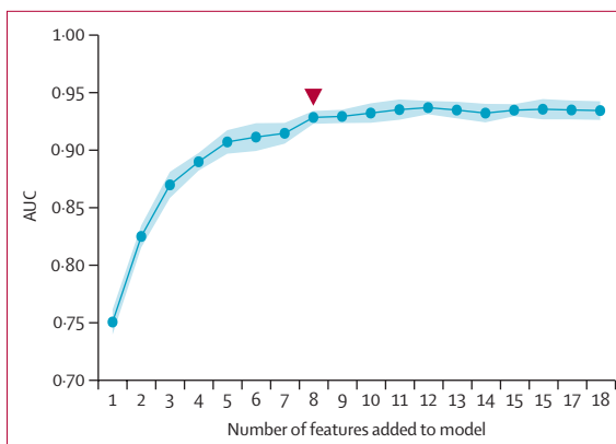
Figure 2: Identification of optimal number of predictive features for a prediction of convulsive epilepsy
