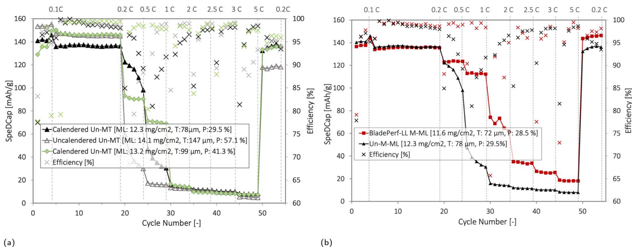
Fig. 9 The specific discharge capacity and coulombic efficiency (%) at different C-rates for lignin/water-based cathodes with medium mass loading ( M-ML = 11.6\text{--}13.2\text{ mg cm}^{-2} ). (a) Compares calendared and uncalendared unstructured (Un) cathodes, and (b) shows how structuring (LL) improves the rate capability of calendared cathodes with low porosity ( P = 28.5\text{--}29.5\% ).
