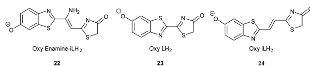
Fig. 6 Deprotonated Oxidized forms of luciferins.
