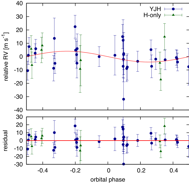
Figure 11. Phase-folded RV curve after subtracting the correlated-noise component via the GP regression. The red solid line represents the best-fit Keplerian orbit of K2-415b, and the bottom panel plots the residuals from the best-fit orbit.
