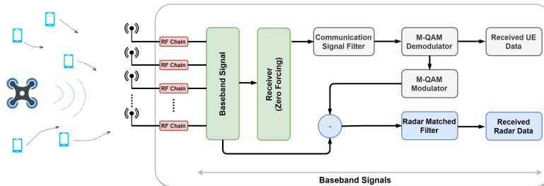
Figure 1: The proposed receiver architecture for a Massive MIMO RadCom system.
