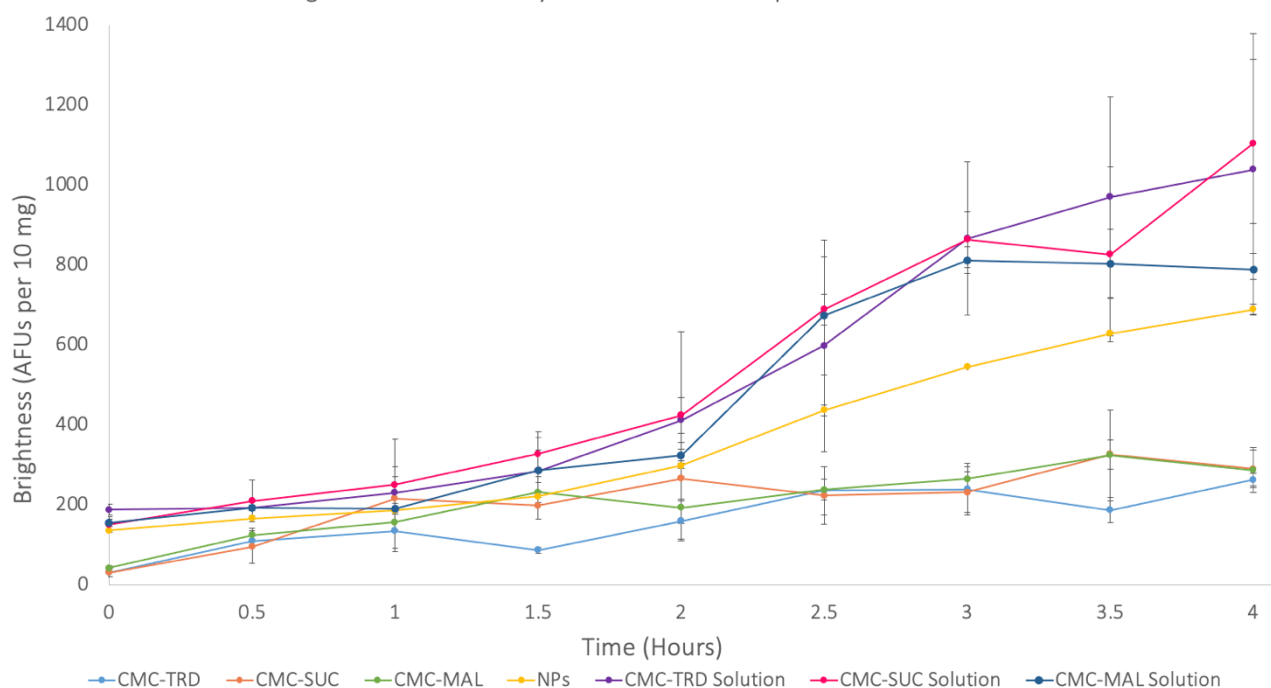
Figure 6 Graph showing the degradation of microneedle arrays with FITC-SiNP encapsulated at 37°C over 4 hours
