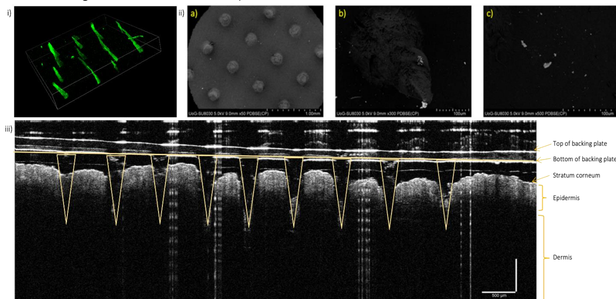
Figure 5 i) Confocal microscopy image of FITC-NP encapsulated into CMC-MAL array; ii) Backscattered SEM images of CMC-MAL microneedle array with AuNP incorporated into the matrix – a) microneedle array with AuNP; b) Single needle of microneedle array with AuNPs incorporated showing an isolated cluster of AuNP on the tip of the needle; c) Backing plate of microneedle array with AuNP showing some aggregated AuNP and some single AuNPs distributed; iii) Optical Coherence Tomography image of biodegradable microneedle array in mouse skin demonstrating the ability of these arrays to penetrate skin without bending or breaking. Yellow colour outlines the position of the individual microneedles.
