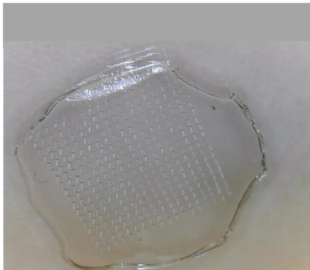
Figure 4 CMC-MAL microneedle array structure consisting of 324 needles of height 750 \mu\text{m} , base diameter 200 \mu\text{m} , tip diameter 10 \mu\text{m} and centre-to-centre spacing of 600 \mu\text{m}
