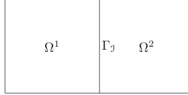
Figure 1: The domain of solution is given by the two subdomains \Omega^1 , \Omega^2 joining at the internal boundary \Gamma_j .
