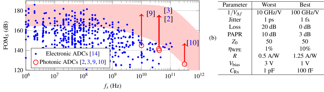
Fig. 3. (a) \text{FOM}_S estimation for photonic ADCs (red circles) compared to published results from electronic ADCs [14]. The red shaded area indicates the achievable \text{FOM}_S for generalised photonic ADCs based on (1)/(2) and the parameters in (b). The red arrows extending from the photonic ADC results indicate the maximum estimated \text{FOM}_S for each architecture.
