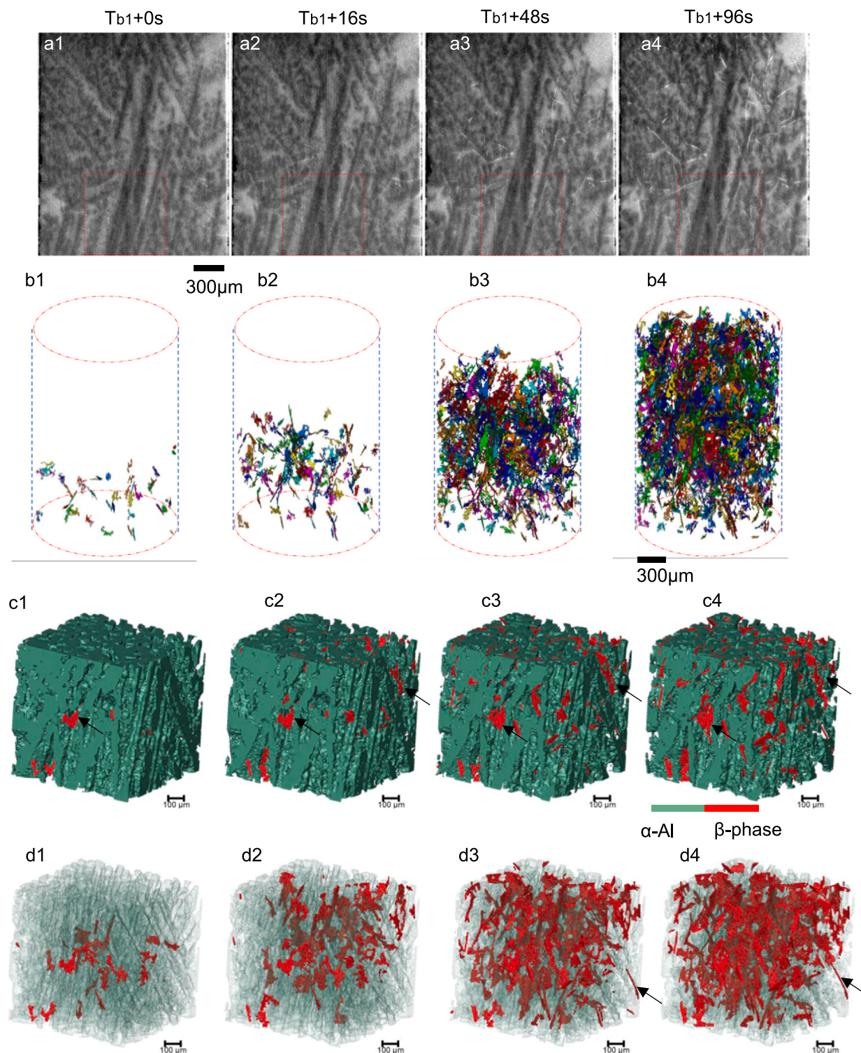
Fig. 4. (a) 2D vertical slices of \beta -phase at different timestamps ( B = 0.5 \text{ T} , TG = 2.5^\circ\text{C/mm} , CR = 0.1^\circ\text{C/s} ); (b) 3D volumes of \beta -phase at different timestamps; Cropped region ( 882 \times 882 \times 882 \mu\text{m}^3 ) from Fig. 3-a at different timestamps (c) 3D volumes (d) 3D volume with transparent \alpha -Al phase.
