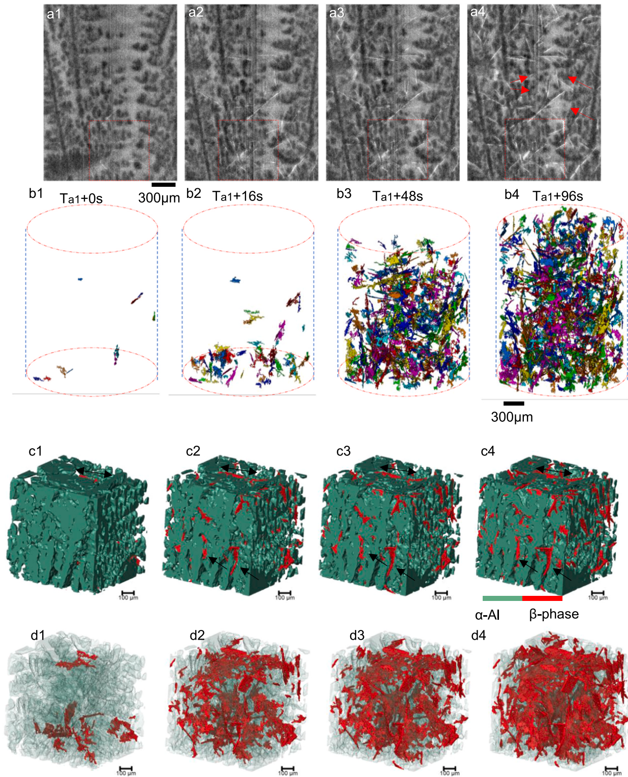
Fig. 3. (a) 2D vertical slices of \beta -phase at different timestamps ( B = 0\text{ T} , T_G = 2.5^\circ\text{C/mm} , CR = 0.1^\circ\text{C/s} ); (b) 3D volumes of \beta -phase at different timestamps; Cropped region ( 882 \times 882 \mu\text{m}^3 ) from Fig. 2-a at different timestamps. (c) 3D volumes (d) 3D volume with transparent \alpha -Al phase.
