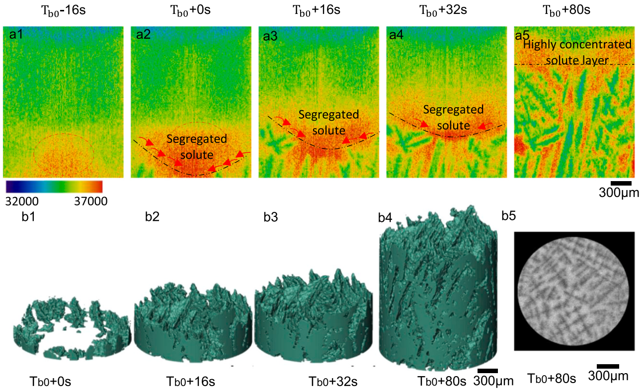
Fig. 2. (a) 2D vertical slices of \alpha -Al phase at different timestamps ( B = 0.5 T, TG = 2.5^\circ\text{C}/\text{mm} , CR = 0.1^\circ\text{C}/\text{s} ); (b1-b4) 3D volumes of \alpha -Al phase at different timestamps; (b5) a horizontal slice at height of 1.1 mm.
