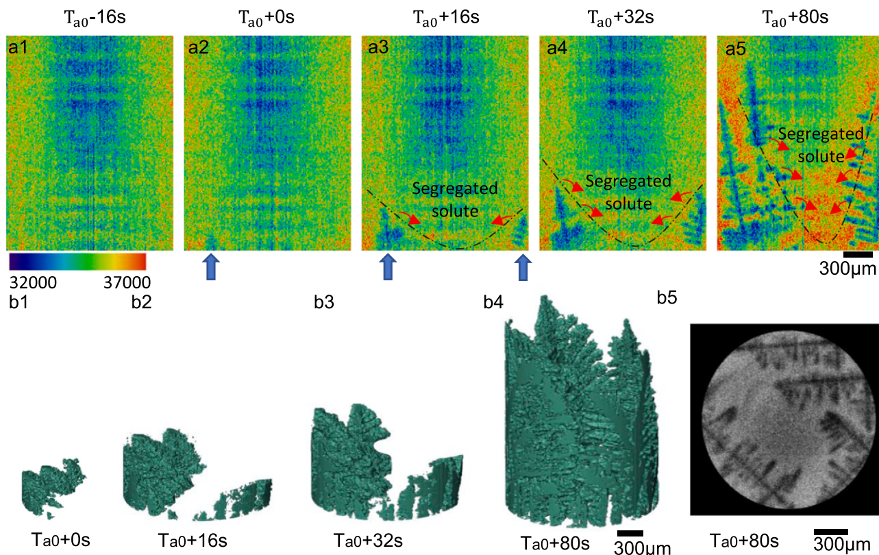
Fig. 1. (a) 2D vertical slices of \alpha -Al phase at different timestamps ( B = 0 T, TG = 2.5 °C/mm, CR = 0.1 °C/s); (b1–b4) 3D volumes of \alpha -Al phase at different timestamps; (b5) a horizontal slice at the height of 1.1 mm.
