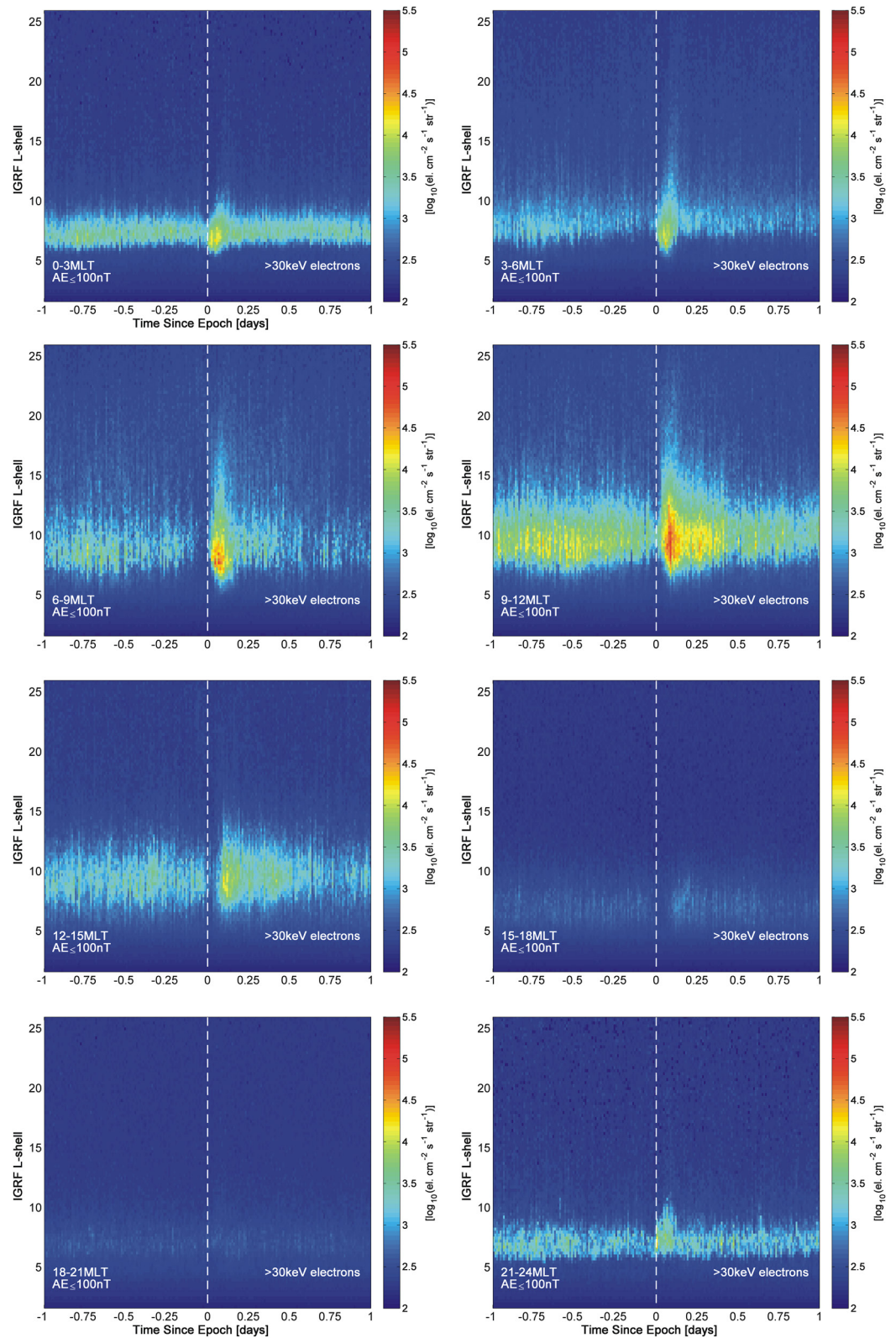
Figure 3. SEA of median >30 keV POES precipitating electrons for the Substorm Cluster Epochs, plotted against L -shell for zero epoch AE values in the range AE \leq 100 nT (i.e., quiet). Each panel is for a different MLT range, as labeled. The format is otherwise as shown in Figure 2.
