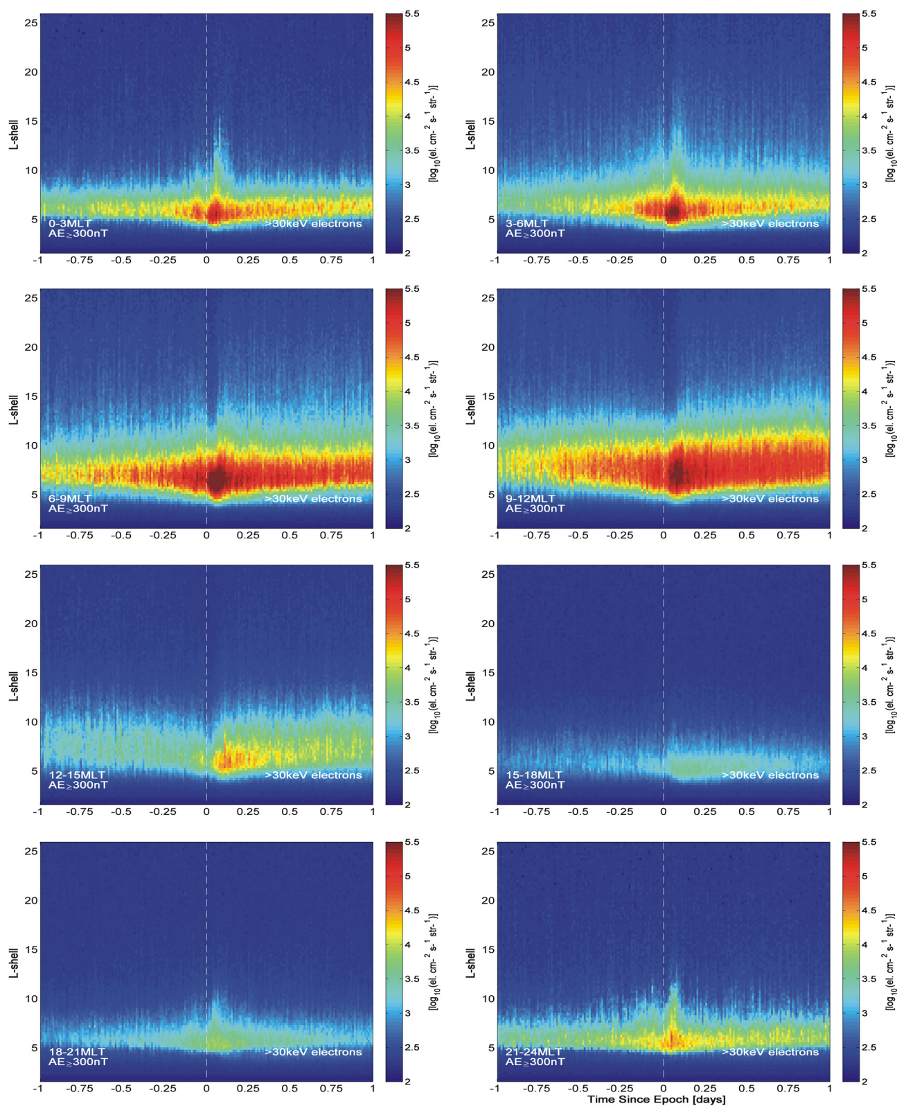
Figure 6. As Figures 3 and 4, but for the strong AE geomagnetic disturbance range ( AE \geq 300\text{ nT} ).
