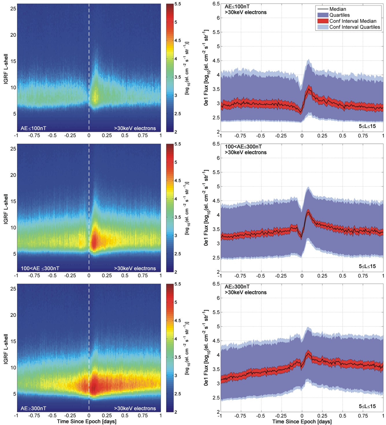
Figure 1. SEA showing the dynamics of the median >30 keV precipitating electron flux variation from POES. The SEA is considered separately for three geomagnetic activity levels, specified by AE index value at the time of zero epoch, which is the start of the substorm cluster. The left hand plots show the SEA of median precipitating electrons for the AE dependent recurrent Substorm Epochs, plotted against L -shell. The right hand plots show the statistical variation of the outer radiation belt >30 keV fluxes in the L -shell range from 5.0 to 15.0. In the right hand panels the superposed epoch median of the plotted parameter is given by the solid black line. The 95% confidence interval for this median is shown by the red band. The dark blue bands mark the interquartile range and the 95% confidence interval about it (light blue).
