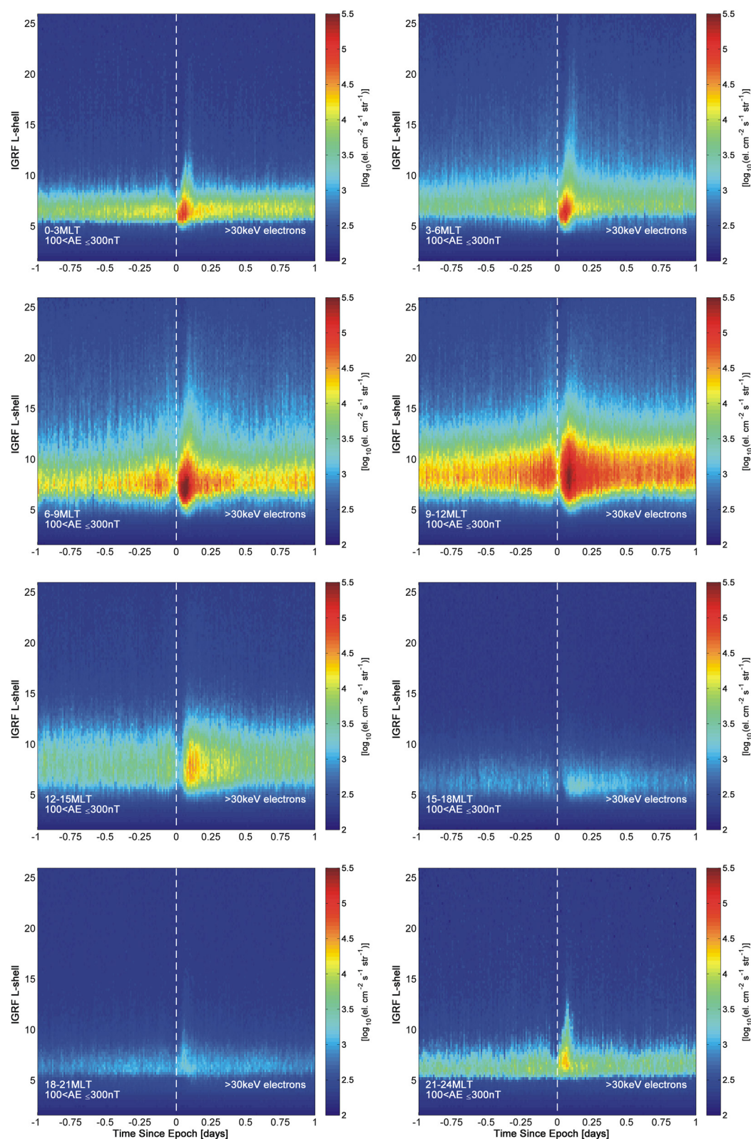
Figure 4. As Figure 3, but for the moderate AE range ( 100 \text{ nT} < \text{AE} \leq 300 \text{ nT} ).
