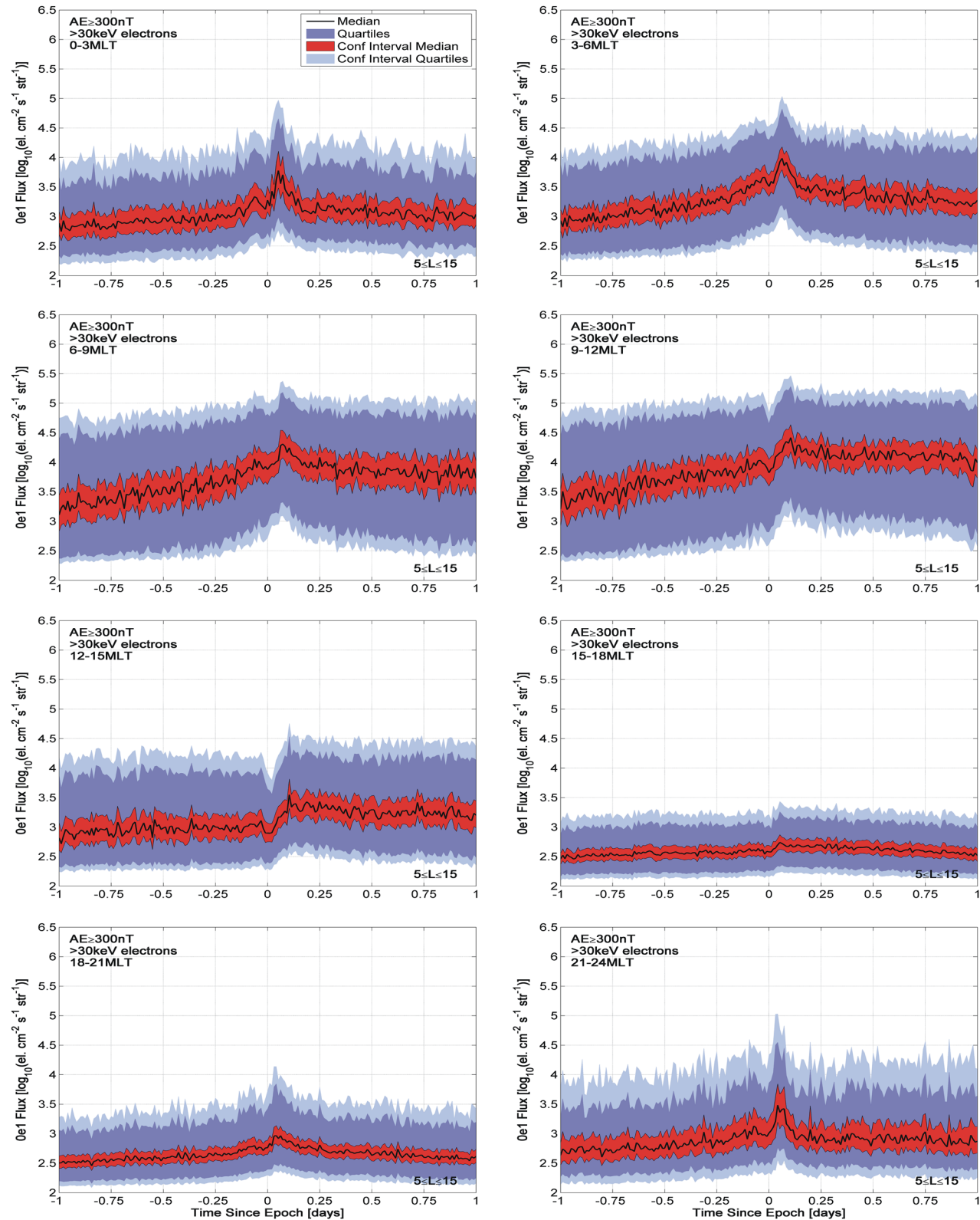
Figure 7. Statistical variation of the >30 keV precipitating fluxes in the L -shell range from 5.0 to 15.0 for the flux variations shown in Figure 6 (i.e., zero epoch AE values in the range \geq 300 n). This figure is in the same format as Figure 5 and the right hand panels of Figure 1.
