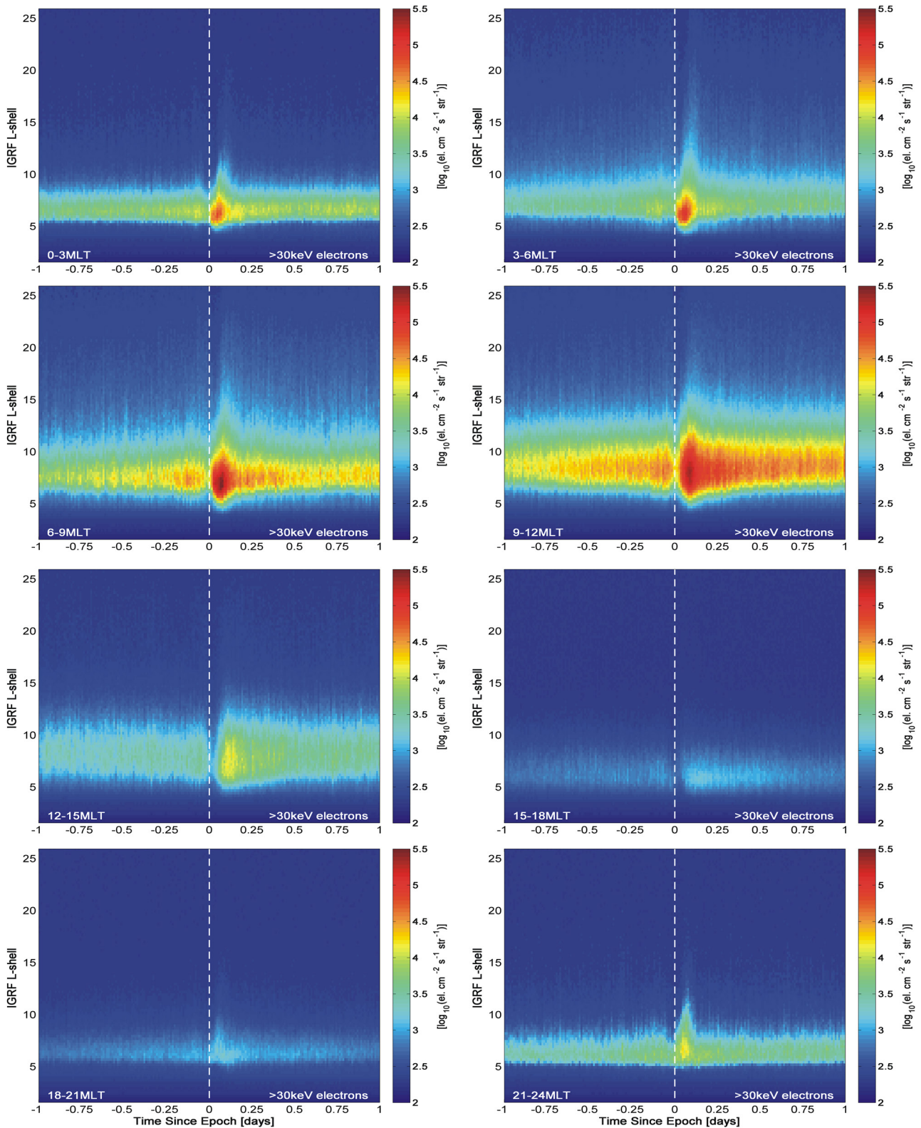
Figure 2. SEA showing the dynamics of the median >30 keV precipitating electron flux variation observed from POES, plotted against L -shell. The start of the substorm cluster defines the zero epoch, shown by the dashed white line in the panels. Each panel is for a different MLT range, as labeled. Note that electrons drift around the Earth from top-left to bottom-right. This SEA uses all the substorm clusters, without discriminating by AE.
