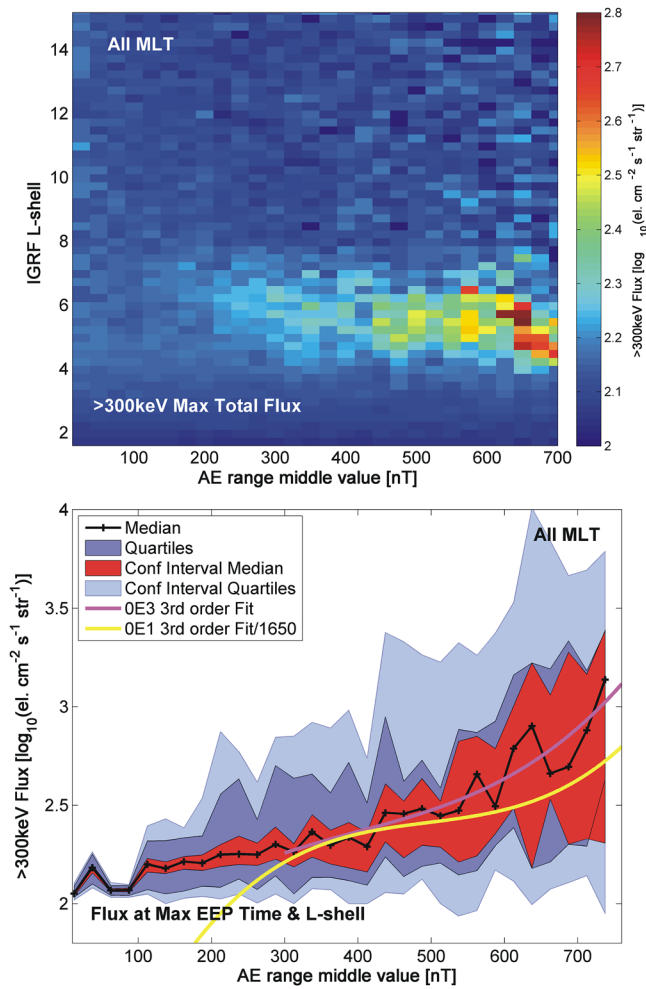
Figure 9. Examination of the variation in peak >300 keV fluxes EEP magnitude with respect to sweeping AE. Top left: L - and AE-variation in 300 keV EEP fluxes at the times where the summed EEP fluxes are maximum for each AE-range. Bottom-left: Statistical variability of the peak >300 keV EEP fluxes, using the same color scales as shown earlier. The magenta line is a 3-order polynomial fit to the median fluxes, while the yellow line is the >30 keV fit shown in Figure 8 divided by 1,650.
