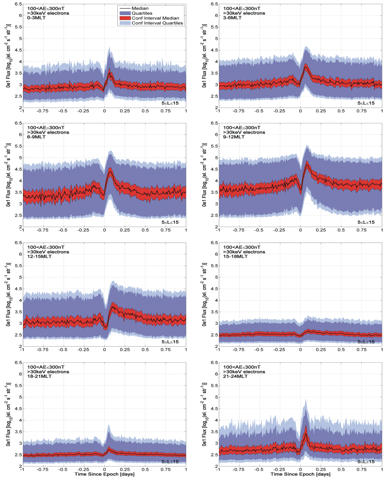
Figure 5. Statistical variation of the >30 keV precipitating fluxes in the L -shell range from 5.0 to 15.0 for the flux variations shown in Figure 4 (i.e., zero epoch AE values in the range 100 \text{ nT} < \text{AE} \leq 300 \text{ nT} ). The median, quartiles, and confidence intervals are plotted in the same format as the right hand panels of Figure 1.
