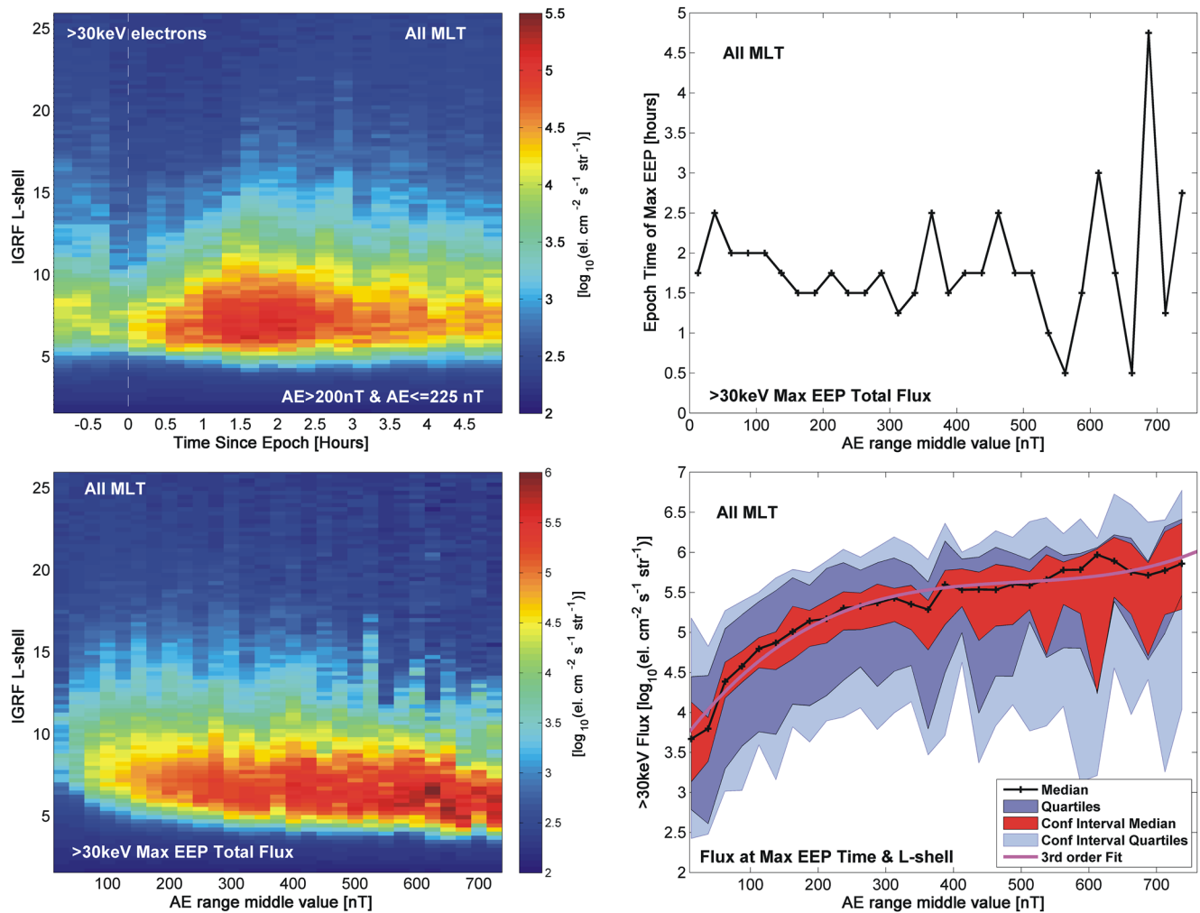
Figure 8. Examination of the variation in peak >30 keV fluxes EEP magnitude with respect to changing AE. Top left: SEA of the >30 keV EEP for the AE range from 200 to 225 nT. Bottom left: L - and AE-variation in 30 keV EEP fluxes at the times where the summed EEP fluxes are maximum for each AE-range. Top-right: Variation in epoch time when the summed EEP fluxes are maximum. Bottom-left: Statistical variability of the peak >30 keV EEP fluxes, using the same color scales as shown earlier (e.g., Figure 3). The magenta line is a 3-order polynomial fit to the median fluxes.
