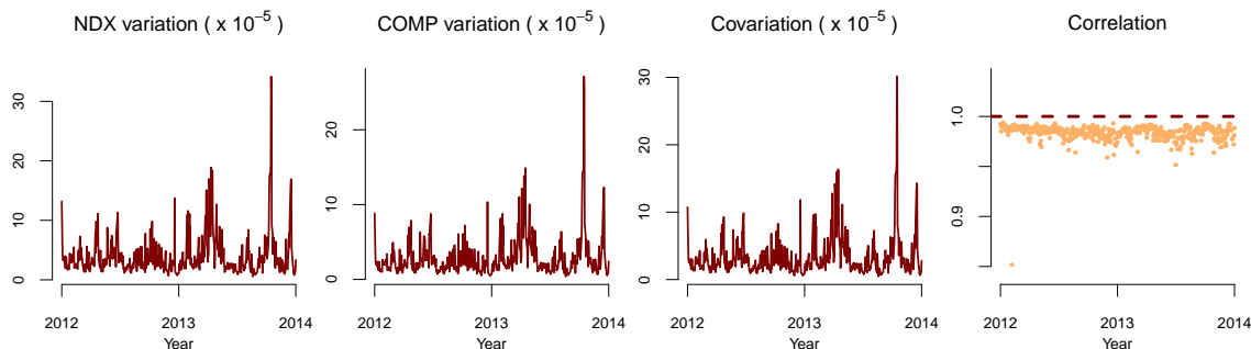
Figure 7: Time series of estimated covariance matrices based on the price of two indices NDX and COMP. Estimated correlations between indices are also plotted against time (red dashed line indicates correlation 1).
