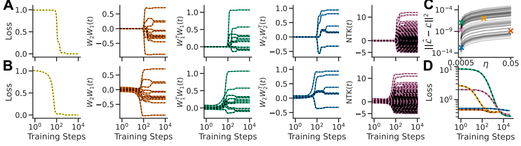
Figure 2: Exact learning dynamics A The temporal dynamics of the numerical simulation (coloured lines) of the loss, network function, correlation of input and output weights and the NTK (columns 1-5 respectively) are exactly matched by the analytical solution (black dotted lines) for small initial weight values and B large initial weight values. C Each line shows the deviation of the analytical loss \hat{\mathcal{L}} from the numerical loss \mathcal{L} for one of n = 50 networks with random architecture and training data (details in Appendix H) across a range of learning rates \eta \in [0.05, 0.0005] . The deviation mutually decreases with the learning rate. D Numerical and analytical learning curves for five randomly sampled example networks (coloured x in C).
