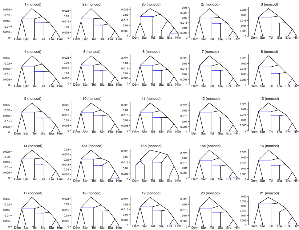
Figure 5. Estimated introgression history of each chromosomal region from noncoding loci. Thickness of the horizontal edges is proportional to the introgression probability estimate. The y-axis is the divergence time. See Figure S4 for the results for coding loci.
