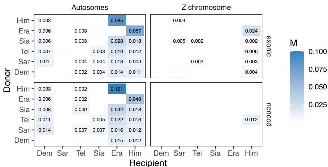
Figure 2. Pairwise migration rate estimates ( M = Nm ) under the IM model from 3s using coding and noncoding loci in the autosomes (using all autosomal loci) and Z chromosome. For each pairwise comparison, the donor and recipient species are given in the y- and x-axis, respectively. H.
