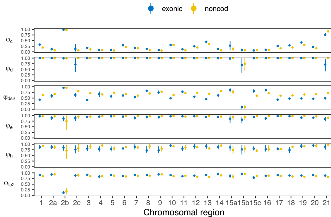
Figure 4. Estimates (posterior mean with 95% HPD interval) of introgression probabilities ( \varphi ) under the model of Figure 3 .
