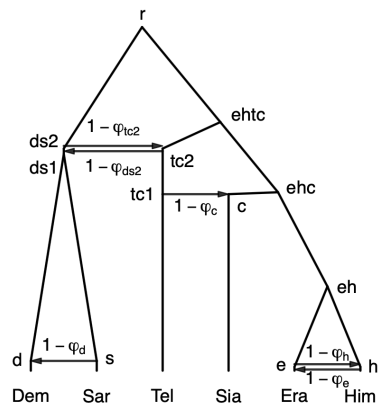
Figure 3. Introgression model. Each horizontal arrow represents a unidirectional introgression event. Timescale drawn here is based on the estimates from all 6,030 noncoding loci in chromosome 1.
