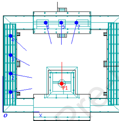
Fig.10. Sound source points to the main hall
