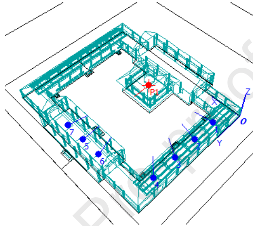
Fig. 2. Sound field model of Jiayintang Theatre
