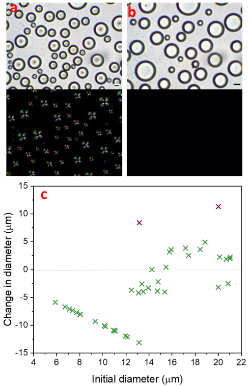
Fig. 1 Nematic droplet size progression over time. Bright-field (Top) and cross-polarised (Bottom) images of 5CB droplets (a) after isotropic-to-nematic transition at -5 °C and (b) after 120 minutes at -5 °C. Scale bar: 10 \mu\text{m} . (c) Change in diameter of droplets between time of isotropic-to-nematic transition point (a) and 120 minutes later (b). Note that the data points coloured in purple relate to droplets that had undergone coalescence.
