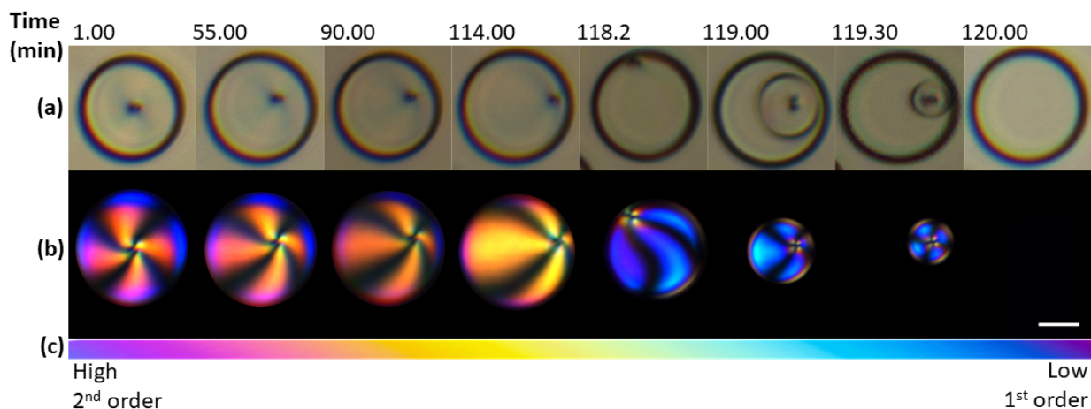
Fig. 2 Birefringence measurements. Evolution of 5CB droplets under (a) Brightfield (b) crossed polarised light over time. (left–right) (c) Colours of the Michel-Levy chart representing decreasing birefringence. The scale bar represents 10\ \mu\text{m} .
