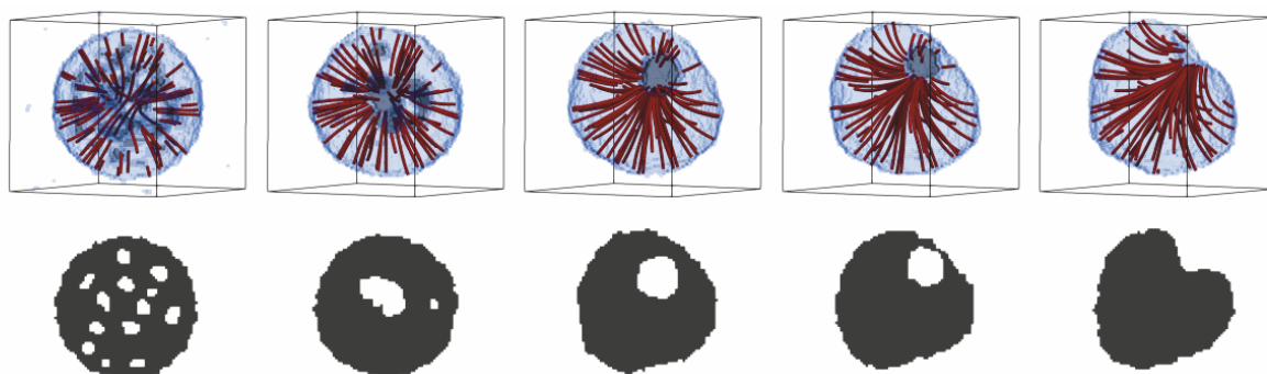
Fig. 3 Defect formation and progression observed through the simulations. The upper images show the LC rich regions (blue) and the LC poor regions inside of the droplet (grey). The red streamlines indicate the local orientation of the nematic LC. The lower images show a cut through the droplet, with LC-rich regions shown in black. From left to right: on initial cooling, the excess solvent deep inside the droplet starts to phase separate at the same time as the anchoring at the interface induces a radial configuration; this evolves to a single small inner droplet at the core of the radial defect; finally the inner droplet touches the exterior and the defect has a escaped radial configuration.
