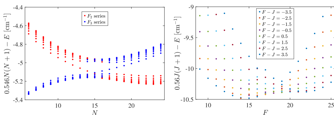
FIG. 9. The left-hand panel shows the avoided crossing structure of the F_2 and F_3 levels of X^4\Sigma^- . Note that, Duo does not use the quantum number N . N is given here simply for the clarity of the figure and was obtained using the rule N = J - 0.5 for the F_2 series and N = J + 0.5 for the F_3 series.
