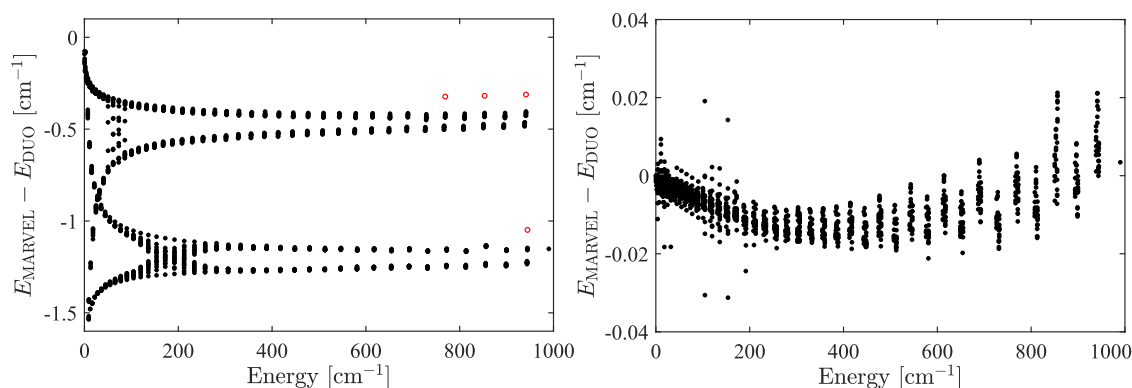
FIG. 8. Energy differences between results of DUO and MARVEL analysis when using ab initio curves. Left: only the R_e value of X^4\Sigma^- was shifted to give correct rotational constants. Right: several other curves were also shifted to reproduce the coupling constants given in Table IV of Flory and Ziurys. 22
