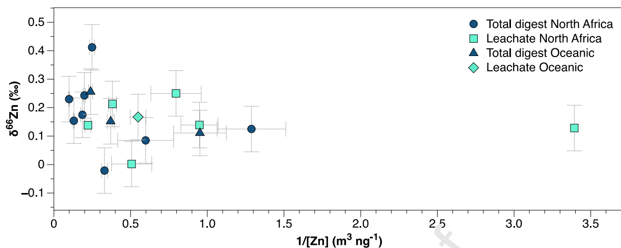
Figure 2: Zn isotope compositions ( \delta^{66}\text{Zn}_{\text{JMC}} ) plotted versus the inverse of atmospheric Zn concentrations ( 1/[\text{Zn}] ). For clarity, the large uncertainty ( \pm 3.3 \text{ m}^3 \text{ng}^{-1} ) associated with the data point with the highest 1/[\text{Zn}] value of 3.4 \text{ m}^3 \text{ng}^{-1} is not shown.
