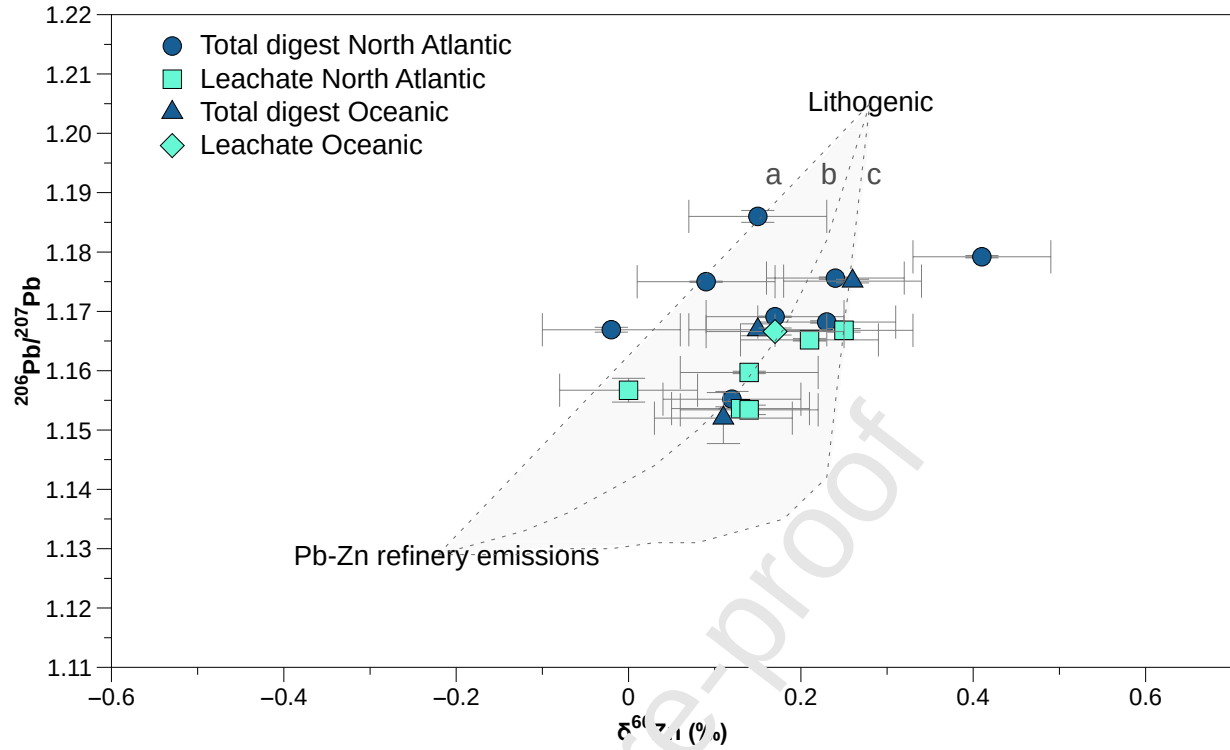
Figure 7: Aerosol Zn isotope compositions plotted against their ^{206}\text{Pb}/^{207}\text{Pb} isotope ratios (Bridgestock et al. 2016). Lithogenic values obtained from Munnich et al., (2017) for Zn ( +0.28 \pm 0.12\text{‰} ) and Bridgestock, (2015; and references therein) for Pb ( 1.20504 \pm 0.00458 ). Pb-Zn refinery emissions from Mattielli et al., (2009) for Zn ( -0.22 \pm 0.34\text{‰} ) and (Cloquet et al., 2006b) for Pb ( 1.1289 \pm 0.0022 ). The dashed lines labelled 'a', 'b' and 'c' are different, hypothetical, mixing lines. 'a' assumes equal parts Zn and Pb from the anthropogenic and lithogenic endmembers. 'b' and 'c' utilise a lithogenic Zn to Pb ratio of 3.94 (equivalent to UCC) and anthropogenic endmember Zn:Pb ratios of 1 for 'b' and 0.09 for 'c' (Cloquet et al., 2006b; Mattielli et al., 2009).
