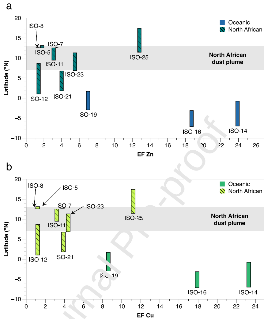
Figure 4: a) Zn enrichment factors plotted against latitude b) Cu enrichment factors plotted against latitude. Both include a grey bar indicating the latitudinal position of the North African dust plume (Bridgestock et al., 2015)
