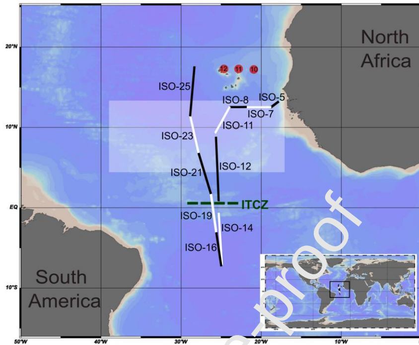
Figure 1: Map of aerosol sampling locations from the GEOTRACES GA06 section cruise (D361, February–March 2011). The white and black marks indicate the distance the aerosols were collected over. The semi-transparent white square represents the approximate region of the North African dust plume at the time of collection (Bridgestock et al., 2016) and the dashed line represents the approximate location of the ITCZ (Schlosser et al., 2014). The red circles labelled 10, 11 and 12 are station locations from the GEOTRACES GA03 cruise (Conway and Johnson, 2014). Schlitzer, R., Ocean Data View, http://odv.awi.de , 2016.
