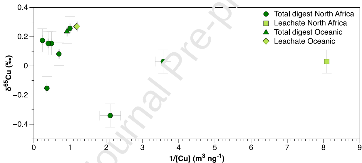
Figure 3: Cu isotope compositions ( \delta^{65}\text{Cu}_{\text{NIST}} ) plotted versus the inverse of atmospheric Cu concentrations ( 1/[\text{Cu}] ). For clarity, the large uncertainty ( \pm 3.1 \text{ m}^3 \text{ng}^{-1} ) associated with the data point with the highest 1/[\text{Cu}] value of 8.1 \text{ m}^3 \text{ng}^{-1} is not shown.
