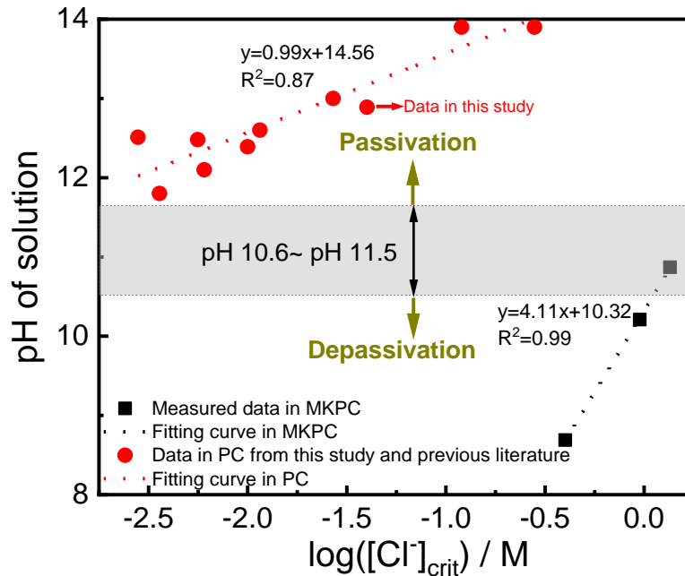
Fig. 12. Comparison between the critical chloride values in MKPC and those in PC, as a function of pH (The data for PC were obtained from this study and the previous literature [22, 51, 95, 96])
