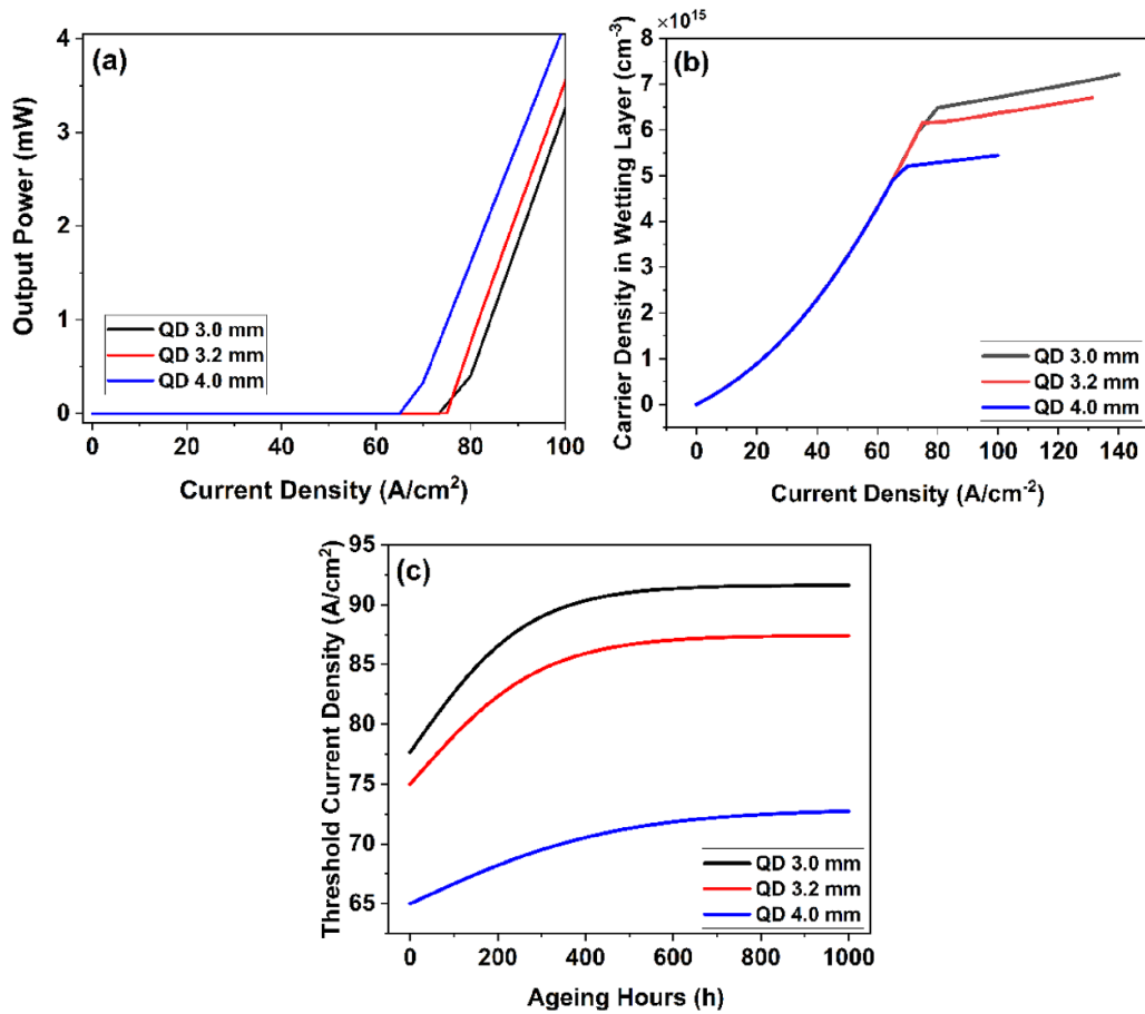
Figure 4. (a) L - I characteristic simulations of QD lasers of different length before the ageing test. (b) Carrier density in WL versus input current density simulations of QD lasers of different length. (c) Rate of degradation simulations of QD lasers of different lengths.
