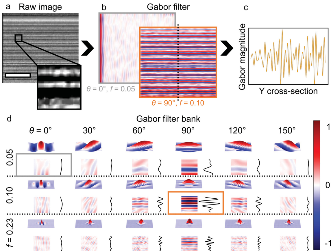
Fig. 1 Directional texture classification using the Gabor filter. (a) A typical X-ray radiography frame captured at 2000 fps showing the electrode layers. The scale bar indicates 1 mm. (b) Images filtered using the Gabor kernel as shown in (d); the electrodes are filtered out when the filter (the sinusoidal harmonic function) is applied perpendicular to the electrodes (radially, \theta = 0^\circ ), whereas the electrode structure is captured when filter is applied parallel to the electrode layers (axially, \theta = 90^\circ ). (c) Y cross-section of the image filtered at \theta = 90^\circ , representing the output of the Gabor filter that is most sensitive to the structure of the electrodes. (d) Gabor kernels with a sinusoidal wavelet (3D projections) applied at varying angles ( \theta ) and frequencies ( f ) on the inset image shown in (a). \theta offers directional sensitivity to selectively filter 'texture' of the electrodes and the frequency ( f ) resolves the individual electrode layers (optimal at f = 0.10 \text{ pixels}^{-1} ). The output signal is maximised for \theta = 90^\circ and f = 0.1 , i.e. , for the filter which best matches the orientation and spacing of the electrodes (orange inset). For filters that do not match with the electrodes, the output signal is reduced, and the texture is not well-represented (grey inset). For an appropriately filtered image, a Gabor signal of +1 represents the Cu/Al layers, -1 that of graphite/electrolyte and values around 0 represent the separator material or the Cu-anode interface/Al-cathode interface.
