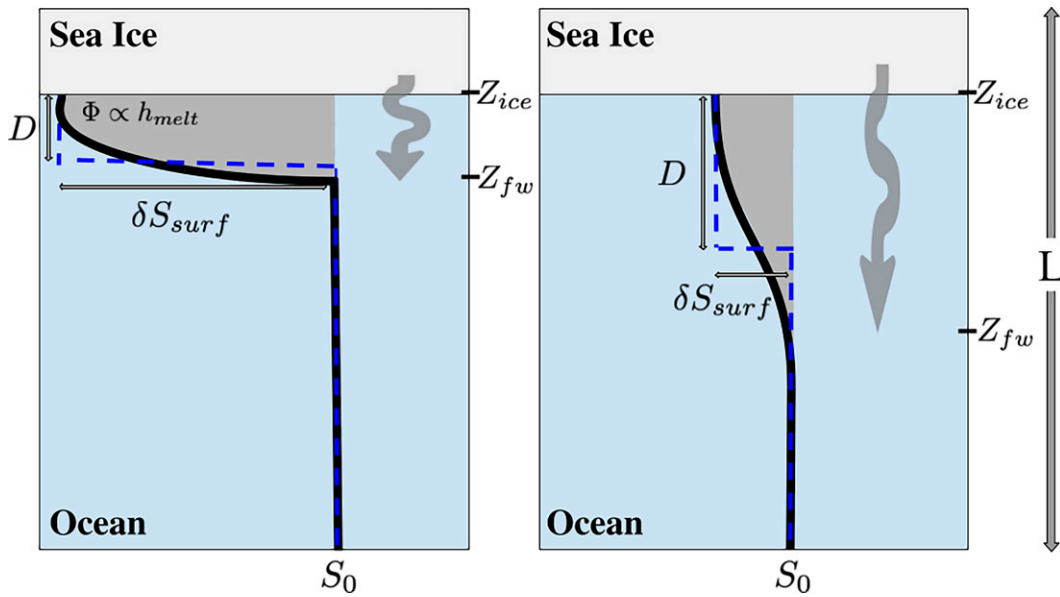
FIG. 2. Schematic of one-dimension ice–ocean model, showing an illustration of the salinity profile resulting from (left) ice melt that is concentrated close to the surface and (right) an example where a similar amount of ice melt is mixed over a larger depth range. Here, L is the depth of the ocean; D , Z_{ice} , and Z_{fw} are negative values that indicate depths; S_0 and \delta S_{surf} indicate the initial salinity and surface freshening, respectively. Area covered by gray shading is equal to \Phi and linearly related to the equivalent sea ice melt ( h_{melt} ). Vertical and horizontal blue dashed lines indicate D and \delta S_{surf} , respectively. Gray arrows represent the vertical extent of sea ice meltwater.
