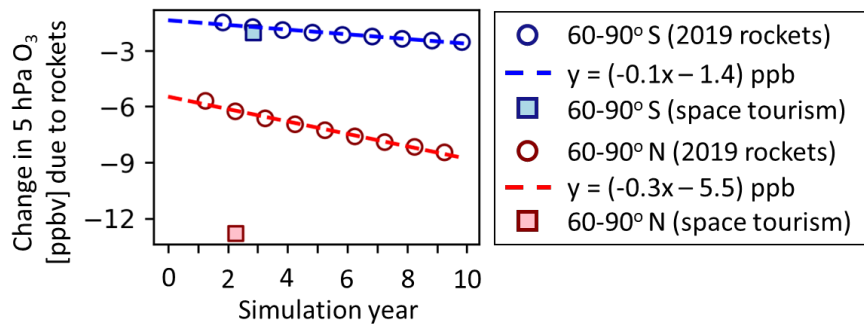
Figure 8. High-latitude springtime upper stratospheric O_3 loss due to rocket launch and re-entry emissions. Open circles show the O_3 response to rocket emissions at 60-90^\circ and 5 hPa altitude for years 2-10 of the decade-long 2019 rocket emissions inventory simulation. Dashed lines show the linear least squares fit to these results. Filled squares show the springtime O_3 loss due to space tourism emissions at the same altitude and latitude range.
