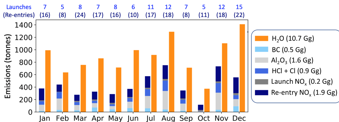
Figure 2. Monthly space sector emissions in 2019 from boosters, first launch stages and re-entry burn as implemented in GEOS-Chem. Numbers in the legend give the total annual emissions of each pollutant. Listed above the chart are the number of launches and re-entries in each month. Emissions increase to 16.7 Gg H 2 O, 0.8 Gg BC, 2.5 Gg Al 2 O 3 , 1.4 Gg HCl + Cl and 3.4 Gg NO x in the last year of the 10-year simulation.
