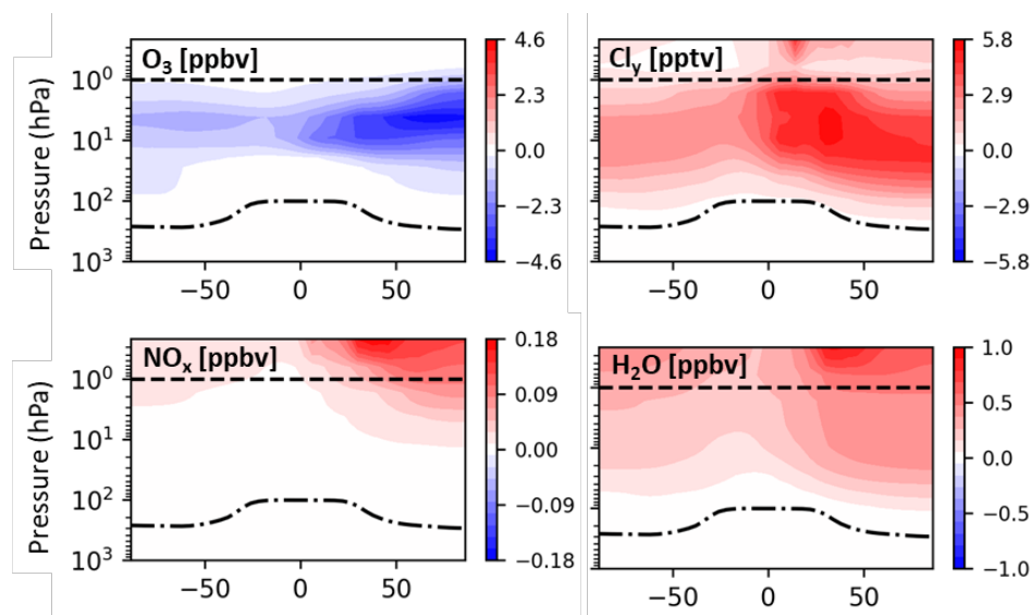
Figure 3. The effect of a decade of sustained growth in rocket and re-entry burn emissions on atmospheric composition. Panels show the change in annual zonal mean mixing ratios of O 3 , Cl y , NO x , and H 2 O due to launch and re-entry ablation emissions.
