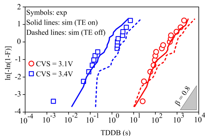
FIG. 5. Comparison between experimental (exp, symbols) and simulated (sim, lines) TDDDB Weibull plots (normalized to 1\mu\text{m}^2 area) of a-HfO 2 MIMs under constant voltage stress (CVS) at 3.1 V (red) and 3.4 V (blue). The simulations are performed for 30 different devices with thermionic emission conduction included (solid lines) and omitted (dashed lines) to demonstrate its impact. All the simulations included the energy correlation of the defect generation process. A slope \beta = 0.8 is shown for reference. The experimental devices and data are described in Ref. 65.
