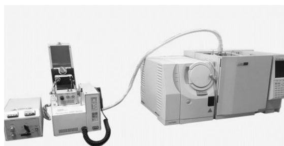
Figure 1: Gas Chromatography and Mass Spectrometry
