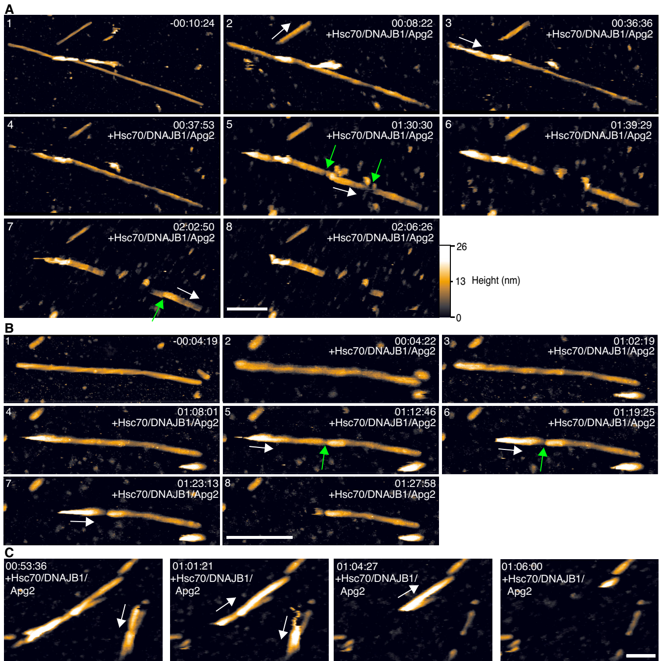
Figure 1. Frames from atomic force microscopy (AFM) movies of \alpha Syn fibre disassembly by Hsc70/DNAJB1/Apg2.
