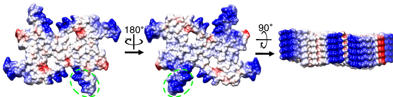
Figure 6. Polarity of the Hsc70 binding site in the ordered part of the fibre structure.
