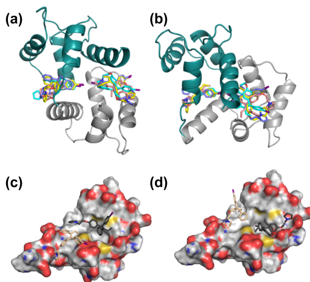
Figure 6. Representative 2 : 1 idoxifene : CaM complex structures. Panels (a) and (b) are orthogonal views of the 2 : 1 idoxifene : CaM complex calculated using NOE-restrained docking of two molecules of idoxifene to CaM coordinates based on the CaM : M13 complex (pdb entry 1cdl). In this calculation, the upper bounds of all observed intermolecular NOEs were set to 5 Å. CaM domains tr1c and tr2c are coloured green and grey respectively and the idoxifene molecules are coloured in pairs (blue, cyan, yellow, or beige) derived from single calculations. View B is orientated to coincide with parts C and D. Panels (c) and (d) show the positions of four molecules of idoxifene derived from a single NOE-restrained docking calculation to the tr2c domain of CaM (from pdb entry 1cll), illustrating one arrangement of four conformations that satisfy the NOE restraints. The four idoxifene molecules are shown in pairs for clarity only. The two darker-coloured idoxifene molecules have either the phenyl group (c) or the p -iodo-phenyl group (d) by the pocket in the hydrophobic surface of the domain. The lighter-coloured molecules also satisfy NOEs that are within reach of the ligand-binding site associated with the tr1c domain. The surface representation of tr2c is coloured as follows: carbon (grey), nitrogen (blue), oxygen (red), and sulfur (yellow).
