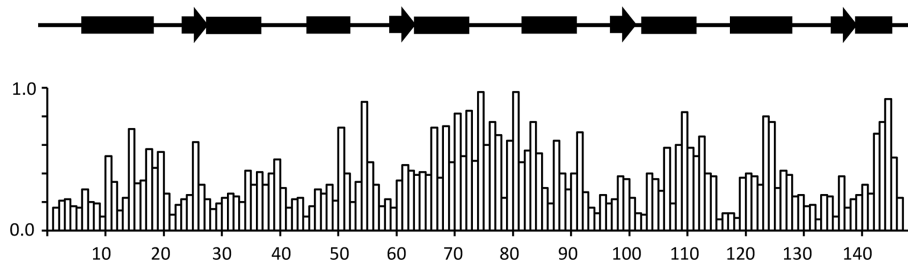
Figure 3. Chemical shift changes for backbone CaM resonances upon binding idoxifene. Normalized, weighted average chemical shift changes are plotted against the primary sequence of CaM. Secondary structure elements are indicated above the histogram as solid boxes for \alpha helices, solid arrows for \beta strands, and thin lines for unstructured regions. The flexible tether (E67–V85) experiences the largest chemical shift changes upon complex formation.
