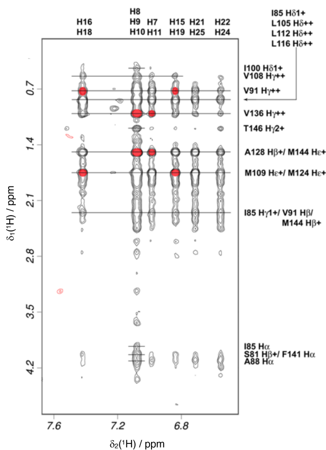
Figure 5. Intermolecular NOEs between idoxifene and CaM. A region of the 2D ^{13}\text{C} - ^{15}\text{N} -double-half-filtered NOESY spectrum of the 2 : 1 idoxifene : CaM complex, processed to exclude the ^{13}\text{C}/^{15}\text{N} bound resonances in the \omega_2 dimension and to include only the ^{13}\text{C} bound resonances in the \omega_1 dimension. The ligand resonances corresponding to each strip are marked on the top edge as follows: p -iodo-phenyl ring (H16/H18), phenyl ring (H8/H9/H10), phenyl ring (H7/H11), p -iodo-phenyl ring (H15/H19), and p -phenoxy ring (H21/H25 and H22/H24). Assignments of the resonances from tr2c are shown on the right. A red circle over the cross peak indicates examples of NOEs that are violated in the structure calculation corresponding to the data in Fig. S3.
