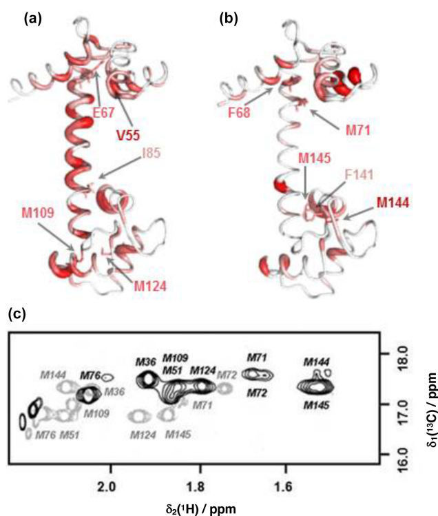
Figure 4. Comparison of backbone and side-chain chemical shift changes in CaM resonances upon binding idoxifene. (a) and (b) : heat map representations of CaM chemical shift changes upon idoxifene binding, shown for clarity using the coordinates of the unliganded CaM X-ray structure, 1c1l. The hydrophobic pocket of the N terminus at the top and the rear of the C-terminal hydrophobic pocket is at the bottom. In (a) residues are coloured according to the weighted average (WA) backbone shift changes observed in the idoxifene : CaM complex, with gradation from white (WA shift = 0.0 ppm) to red (WA shift > 0.7 ppm) and the broadest ribbon indicating the maximum shift changes. The locations of M109 and M124 by the hydrophobic pocket of the C domain are indicated. Residues I85 and E67 are indicated, as they define the central portion of the flexible tether joining the two domains. The position of V55, which undergoes a large shift change as in the CaM : M13 complex, is also indicated. In (b) residues are coloured according to the largest side-chain ^1\text{H} shift changes observed upon idoxifene binding (shifts > 0.50 ppm), with colour gradation and ribbon width depicted as in (a) . The locations of key residues such as three of the nine methionines in the vicinity of the hydrophobic pockets and F68 and F141 are indicated. (c) A 2D ^{13}\text{C} CT-HSQC spectrum showing the \epsilon methyl methionine signals of free CaM (grey) and idoxifene-bound CaM (black).
