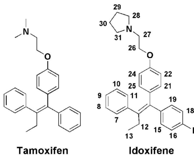
Figure 1. The chemical structures of tamoxifen and idoxifene. The numbering scheme for idoxifene used here is shown: phenyl group: H7–H11; ethyl group: H12–H13; p -iodo-phenyl group: H15–H19; p -phenoxy group: H21–H25; pyrrolidine group: H28–H31.
