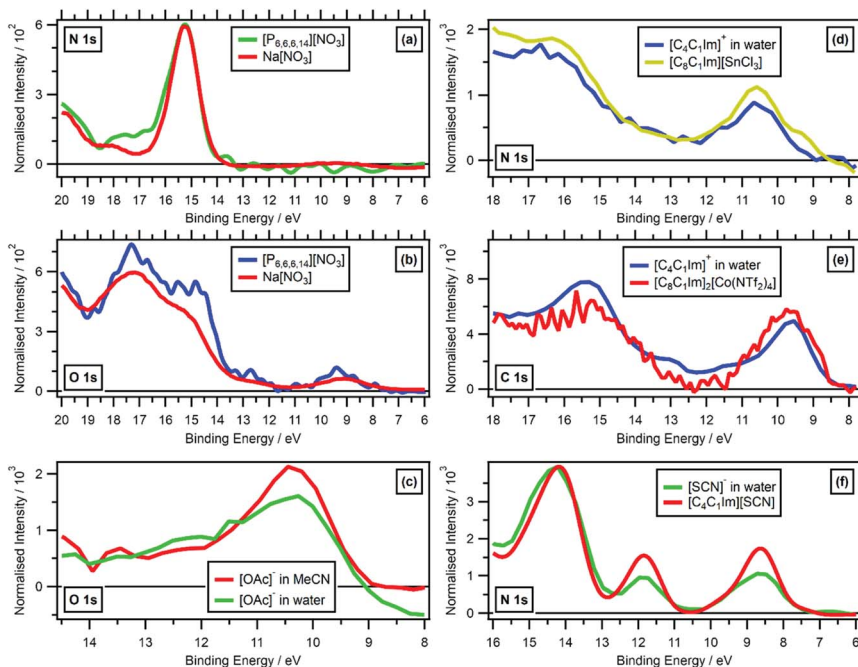
Fig. 8 Valence RXPS traces at different absorption edges. (a) N 1s valence RXPS traces for solid \text{Na}[\text{NO}_3] ( h\nu = 405.0 eV, data from ref. 41) and [\text{P}_{6,6,6,14}][\text{NO}_3] ( h\nu = 405.0 eV). (b) O 1s valence RXPS traces for solid \text{Na}[\text{NO}_3] ( h\nu = 532.0 eV, data from ref. 41) and [\text{P}_{6,6,6,14}][\text{NO}_3] ( h\nu = 405.2 eV). (c) O 1s valence RXPS traces for 1.3 M [\text{C}_4\text{C}_1\text{Im}][\text{OAc}] in water ( h\nu = 532.7 eV) and 0.5 M [\text{C}_4\text{C}_1\text{Im}][\text{OAc}] in MeCN ( h\nu = 532.7 eV). (d) N 1s valence RXPS traces for 0.5 M [\text{C}_4\text{C}_1\text{Im}] in water ( h\nu = 402.1 eV) and [\text{C}_8\text{C}_1\text{Im}][\text{SnCl}_3] ( h\nu = 401.8 eV, data taken from ref. 69). (e) C 1s valence RXPS traces for 0.5 M [\text{C}_4\text{C}_1\text{Im}] in water ( h\nu = 287.0 eV) and [\text{C}_8\text{C}_1\text{Im}]_2[\text{Co}(\text{NTf}_2)_4] ( h\nu = 285.5 eV, data taken from ref. 69). (f) N 1s valence RXPS traces for 0.5 M [\text{C}_4\text{C}_1\text{Im}][\text{SCN}] in water ( h\nu = 399.8 eV) and [\text{C}_4\text{C}_1\text{Im}][\text{SCN}] ( h\nu = 399.5 eV). The valence NRXPS contributions were subtracted using the procedure outlined in ref. 68. All electron spectra were charge referenced using procedures outlined in Section 2.5.
