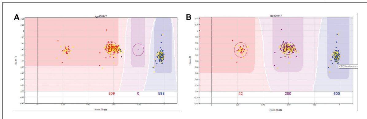
Figure 9 Unexpected cluster position: (A) The AA homozygote cluster has shifted to the right, where the AB cluster is expected, causing the AA homozygote and heterozygote cluster to be classified as AA homozygote. (B) The clusters can be manually moved to correct the misclassification.
