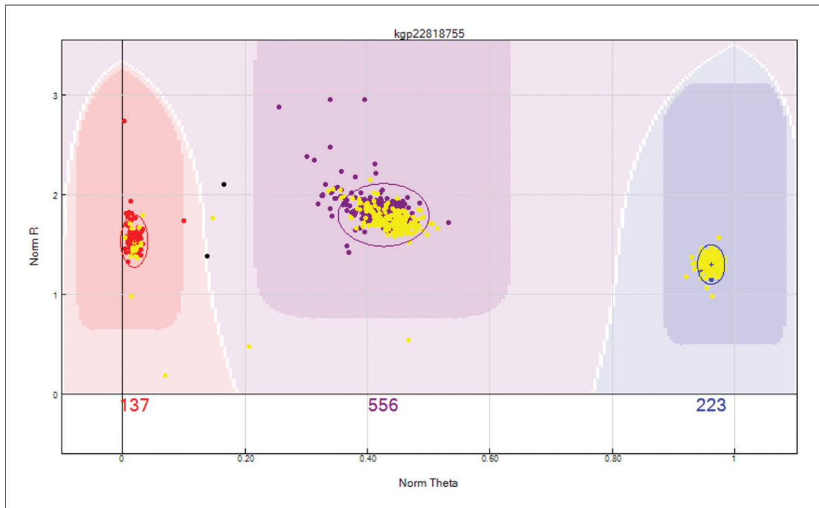
Figure 4 X chromosome unreliable SNP. This X chromosome SNP has female samples highlighted in yellow and male samples are red, purple, or blue depending on their clustering location. Male samples have a single X chromosome and therefore cannot be heterozygote as shown above. If the male samples cannot be manually removed from the heterozygote cluster, then the SNP should be zeroed.
