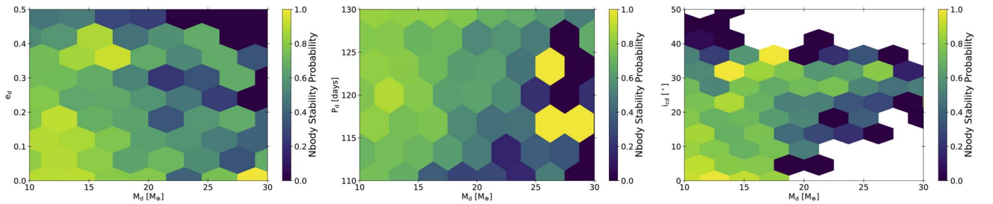
Figure 11. Stability maps for \pi Men d. Yellow and green regions indicate binned values with a high probability of stability whereas dark regions are unstable. (Left) Stability regions in the eccentricity-planet-mass plane. (Middle) Stability regions in the of orbital-period planet-mass plane. (Right) Stability regions in the inclination-planet-mass plane.
