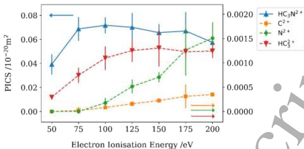
Figure 5 Partial electron ionisation cross sections for the formation of the observed dications following electron ionisation of HC 3 N. The dashed lines are aligned with the right axis as indicated by arrows. See text for details.
