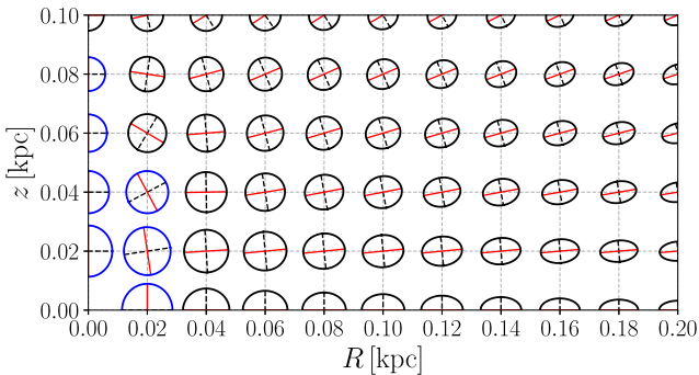
Figure 17. Representation of the velocity ellipsoids of the NSD fiducial model. Red is the major axis of the ellipse, while black dashed is the minor axis. The length of the red axes of each ellipse is proportional to the largest eigenvalues of the velocity ellipsoid at the centre of the ellipse. Blue indicates the ellipsoids that are vertically biased (i.e. the angle between the major axis and the z axis is less than 45^\circ ).
